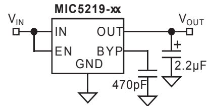
Figure 6. Ultra-Low-Noise Fixed Voltage Regulator
