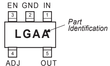
MIC5219BM5 SOT-23-5 Adjustable Voltage (Top View)
