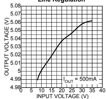
Line Regulation
