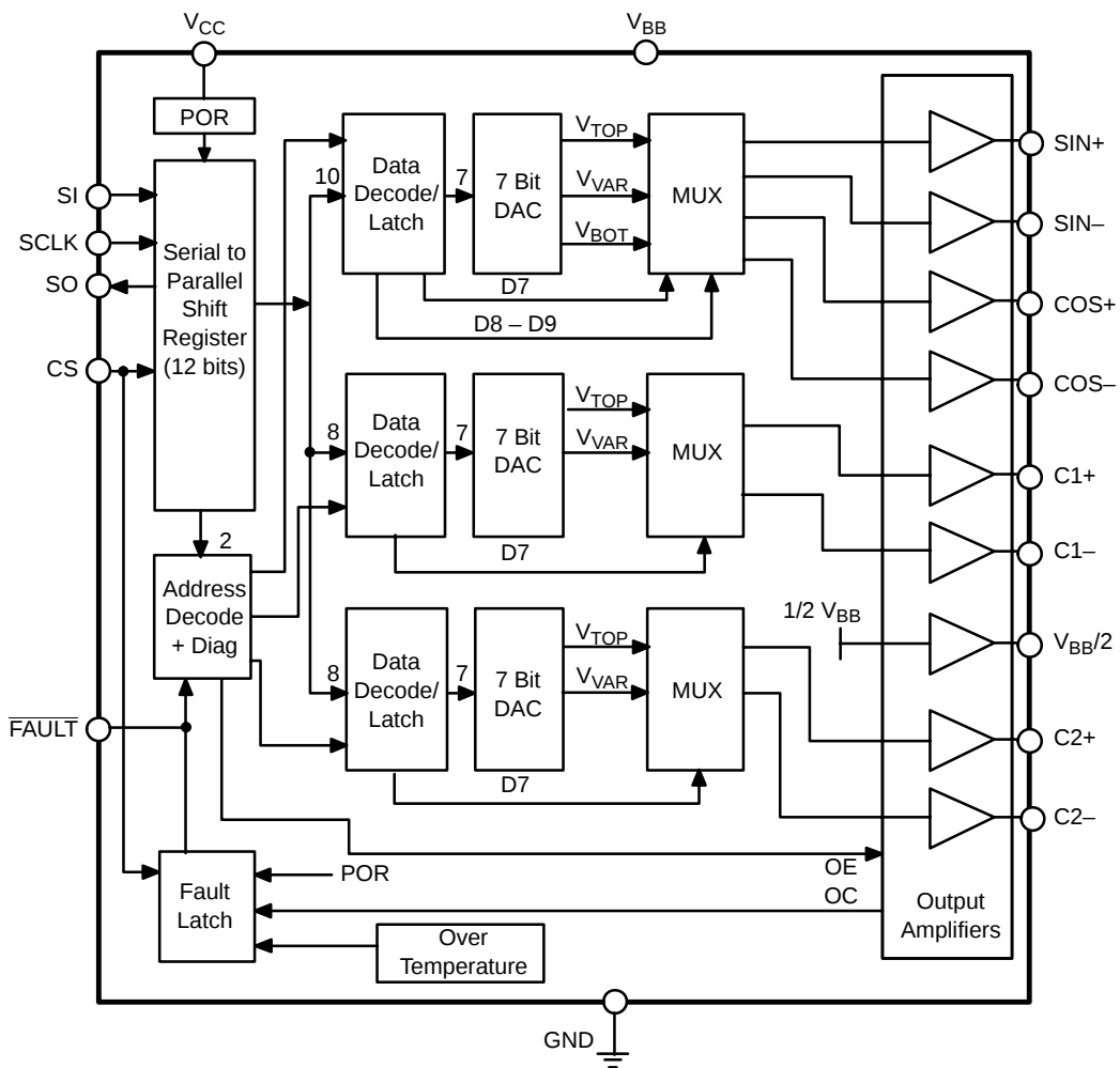
Figure 1. Block Diagram
