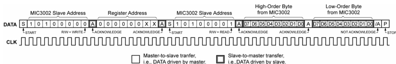
Figure 23. Read Word Protocol
