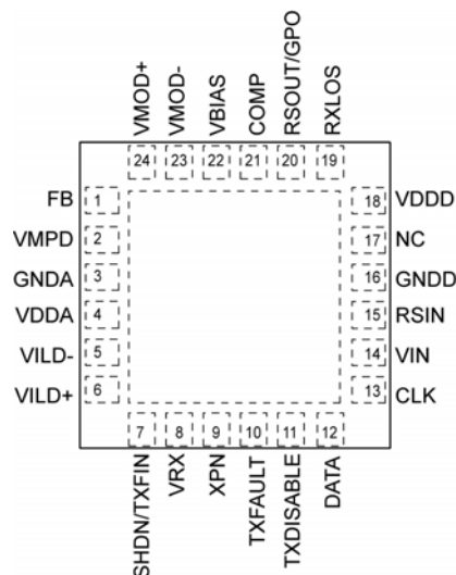
24-Pin MLF ® (MLF-24)
