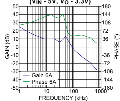
Bode Plot ( V_{IN} - 5V , V_O - 3.3V )
