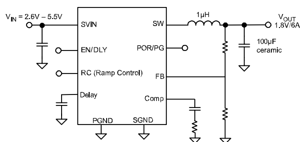
MIC22600 6A 1MHz Synchronous Output Converter
