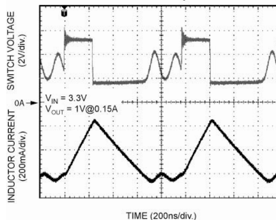
Discontinuous Operation
