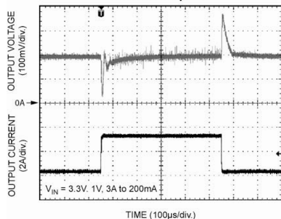
Transient Response
