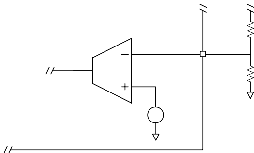
Figure 2. Voltage-Divider Configuration
