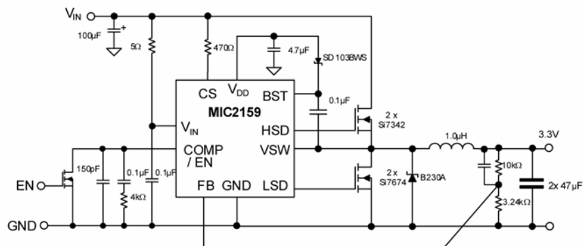
MIC2159 Adjustable Output 400kHz Converter
