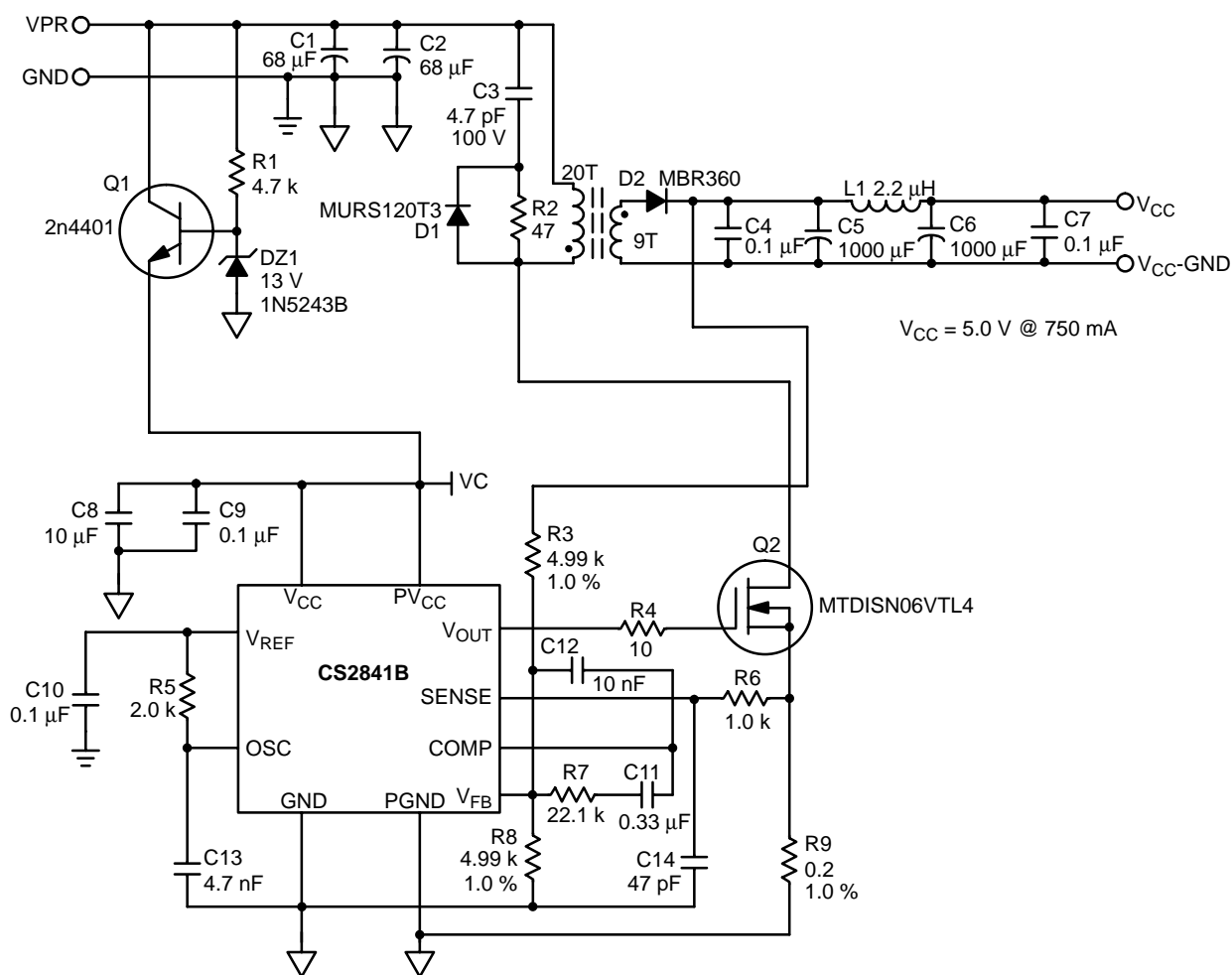
Figure 8. Flyback Application
