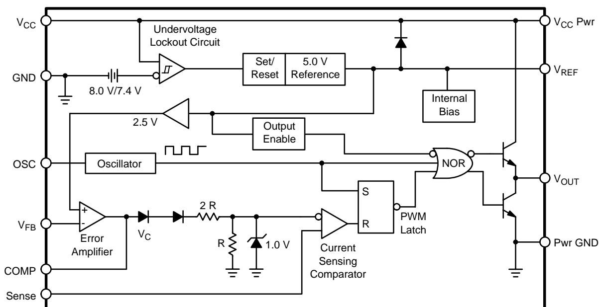
Figure 1. Block Diagram
