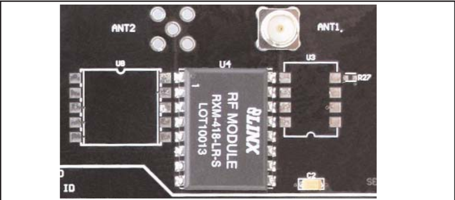
Figure 7: The Decoder Board RF Area
