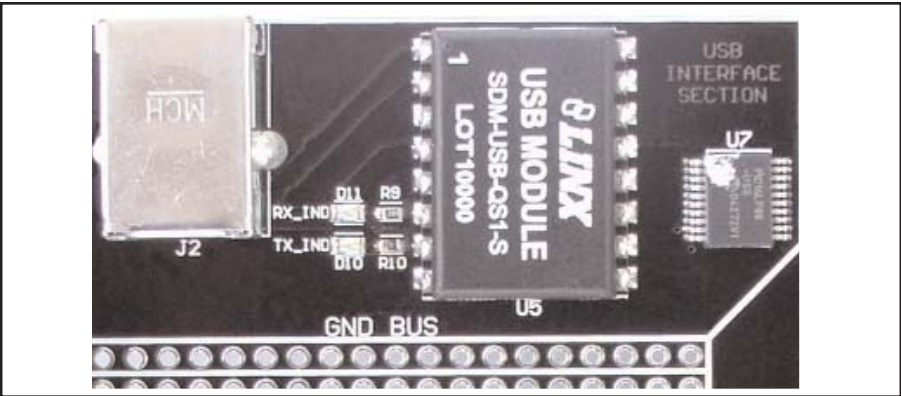
Figure 8: The Decoder Board USB Area
