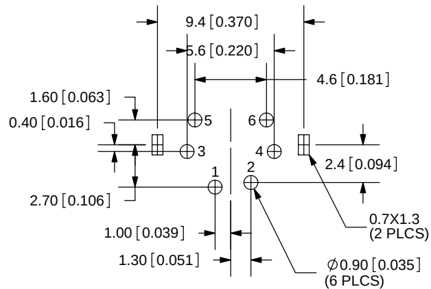
PCB LAYOUT BACK VIEW
