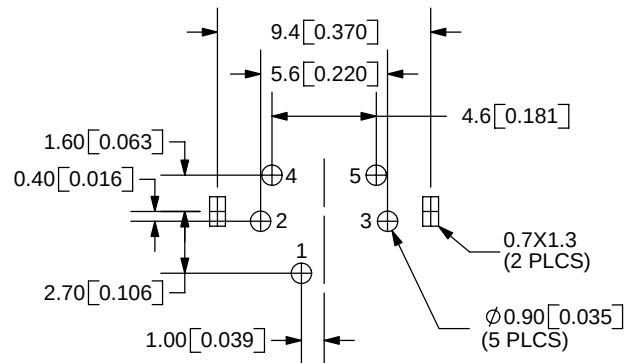
PCB LAYOUT BACK VIEW
