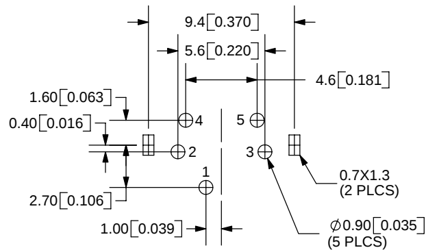
PCB LAYOUT BACK VIEW
