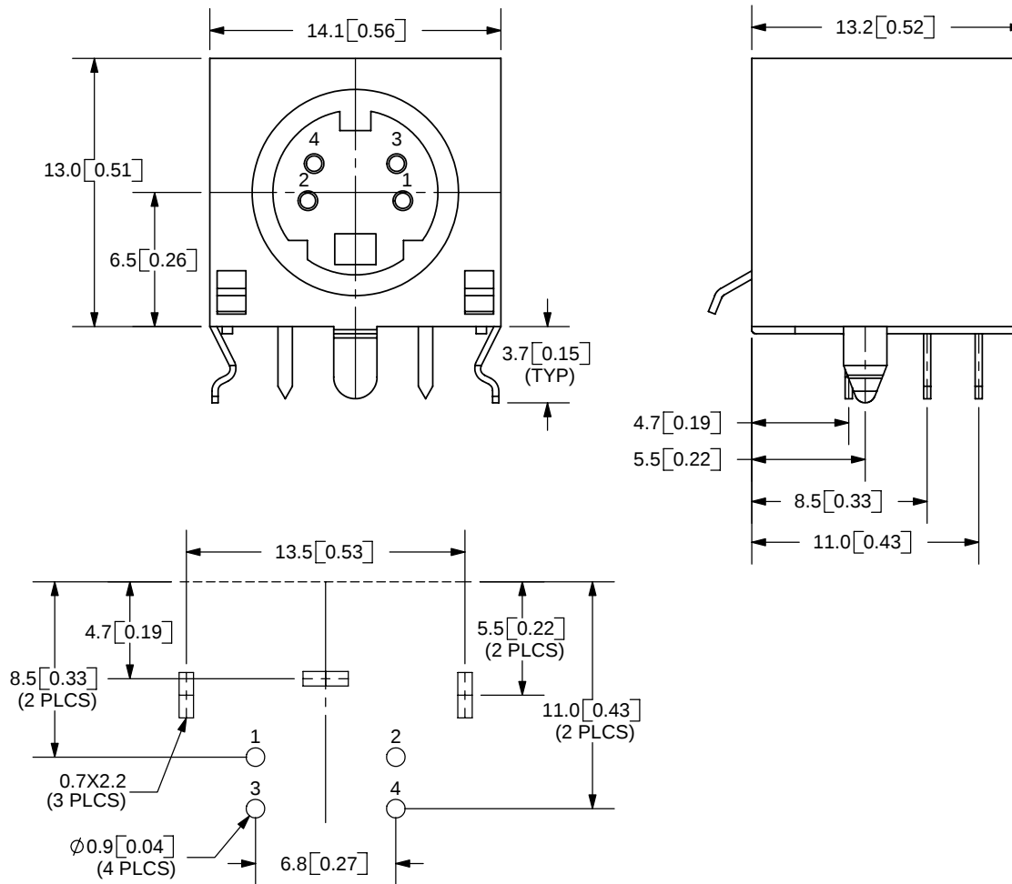
PCB LAYOUT TOP VIEW
