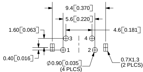
PCB LAYOUT BACK VIEW
