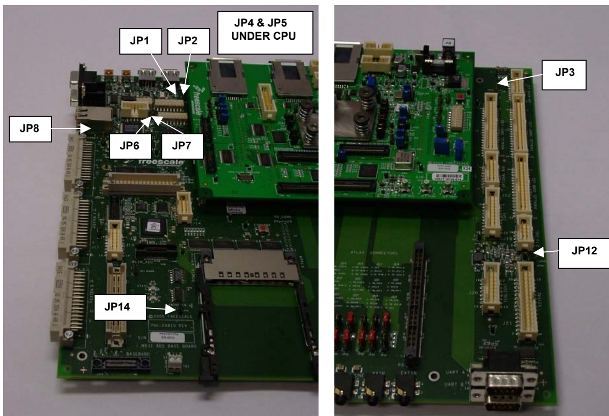
Figure 18. Remaining Baseboard Jumper Configuration
