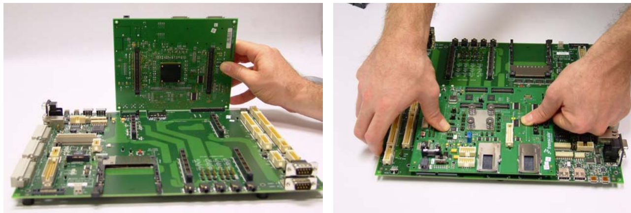
Figure 5. Connecting the CPU to the Baseboard
