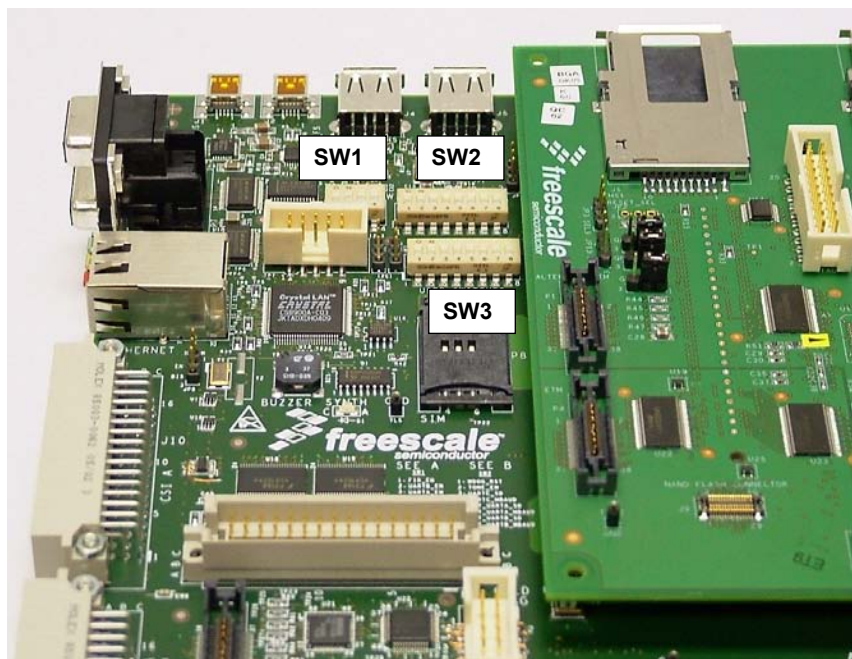
Figure 21. Baseboard Switches
