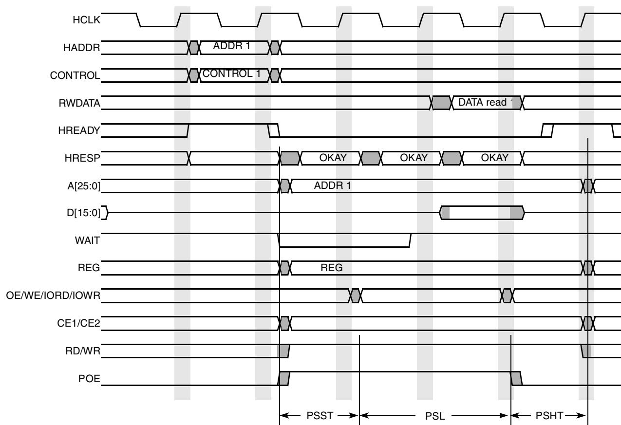
Figure 36. Read Accesses Timing Diagram—PSHT=1, PSST=1
