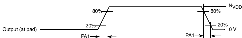
Figure 3. Output Pad Transition Time Waveform
