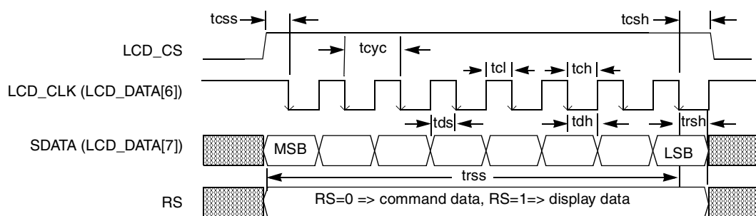
Figure 43. SLCD C Timing Diagram—Serial Transfers to LCD Device
