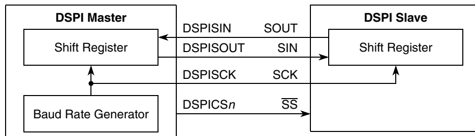
Figure 28-11. SPI Serial Protocol Overview
