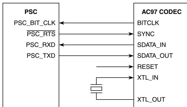
Figure 27-33. An Example Connection to AC97 CODEC
