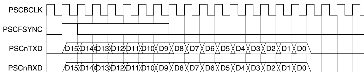
Figure 27-31. Waveform of Modem16 Mode
