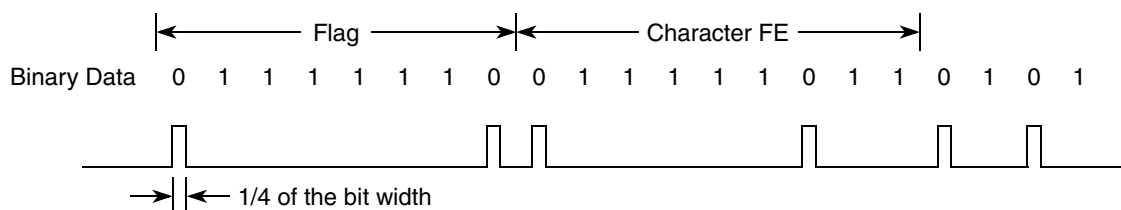
Figure 27-36. Data Format in MIR Mode
