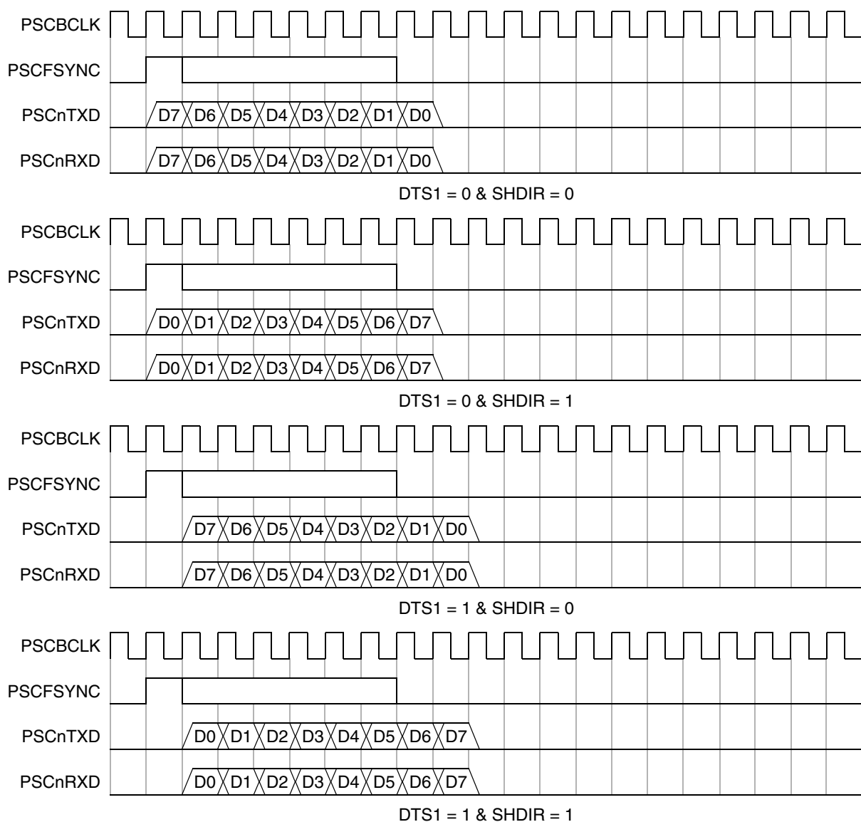
Figure 27-30. Waveform of Modem8 Mode
