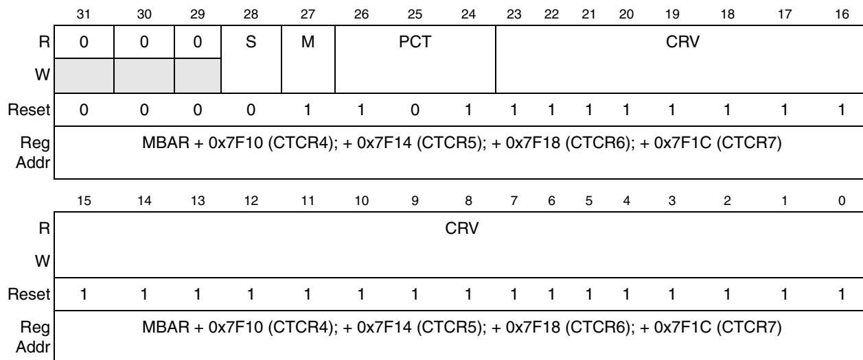
Figure 26-5. Comm Timer Configuration Register (CTCR4-CTCR7) —Variable Timer Channels
