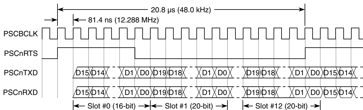
Figure 27-32. Waveform of AC97 Mode
