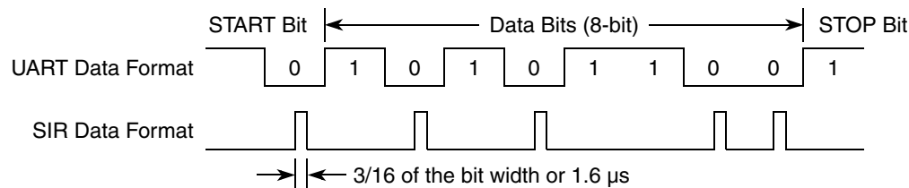
Figure 27-35. Data Format in SIR Mode
