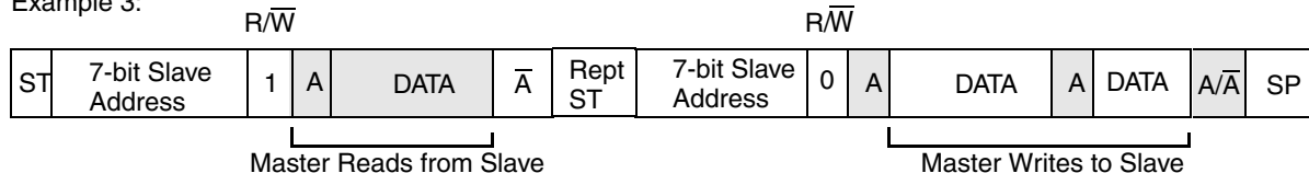
Figure 29-11. Data Transfer, Combined Format
