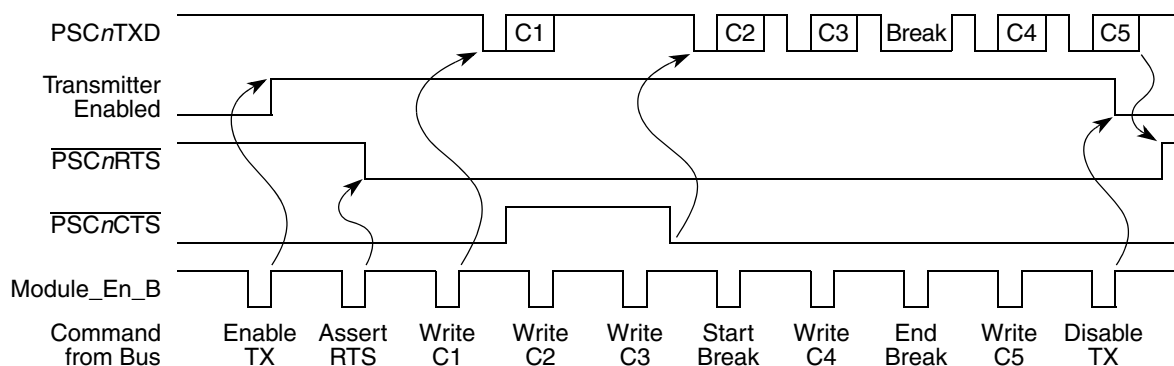
Figure 27-28. Modem Control and Transmitter
