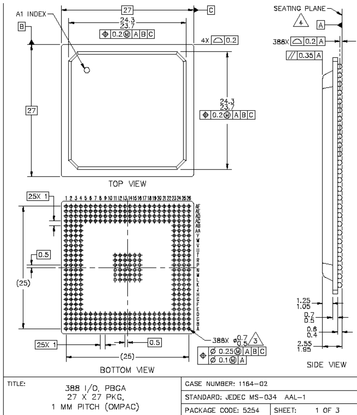
Figure 32-13. 388-pin BGA Case Outline
