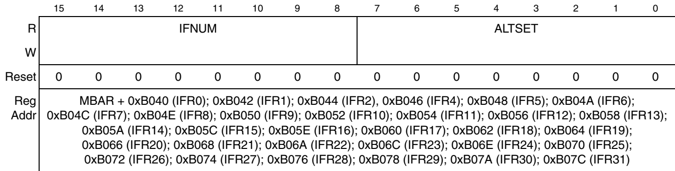
Figure 30-17. USB Configuration Interface Register (IFR n )
