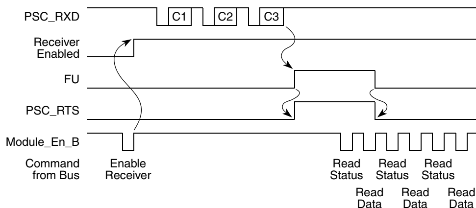
Figure 27-29. Modem Control and Receiver
