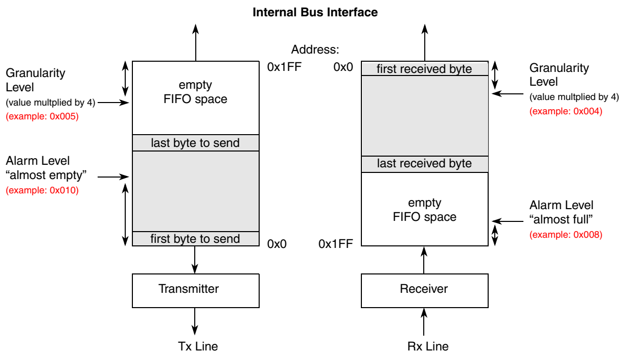
Figure 27-41. PSC FIFO System
