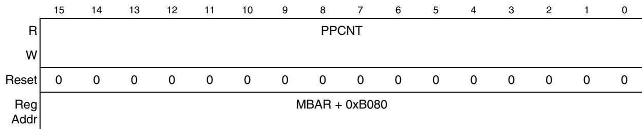
Figure 30-18. USB Packet Passed Count Register (PPCNT)
