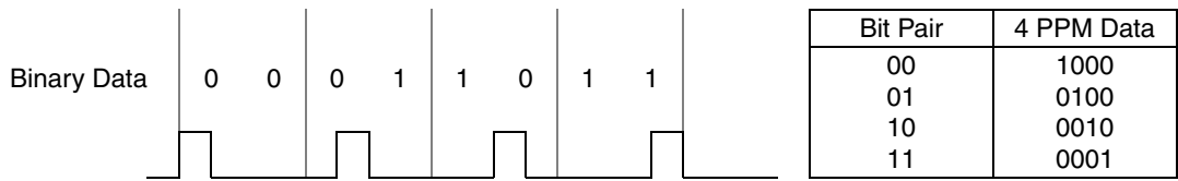
Figure 27-39. Data Format in FIR Mode
