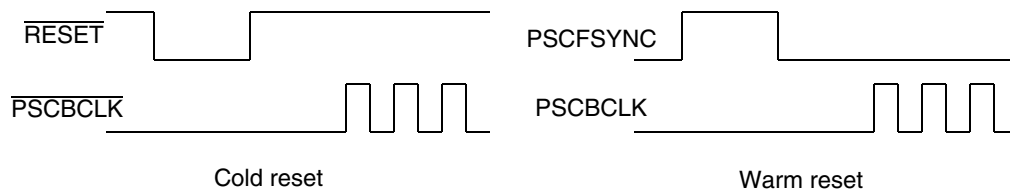
Figure 27-34. AC97 Cold and Warm Reset
