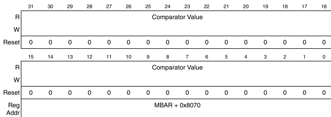
Figure 24-16. Debug Comparator Register (DBGCMP n )
