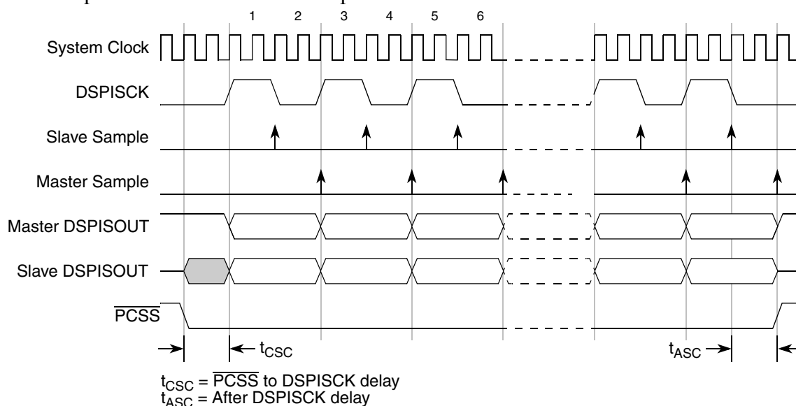
Figure 28-18. DSPI Modified Transfer Format (MTFE = 1, CPHA = 1, Fsk = Fsys/4)
