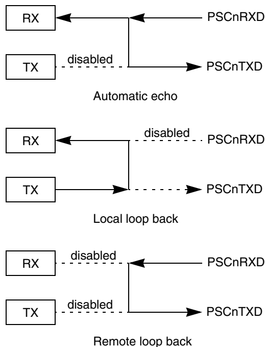
Figure 27-42. Looping Modes Functional Diagram
