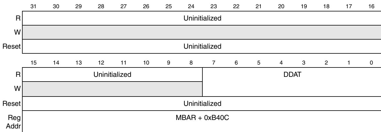
Figure 29-5. USB Descriptor RAM Data Register (DRAMDR)
