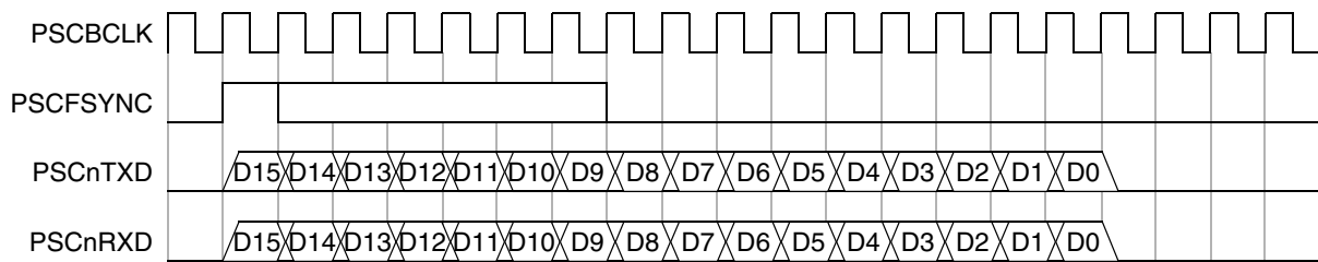
Figure 26-31. Waveform of Modem16 Mode
