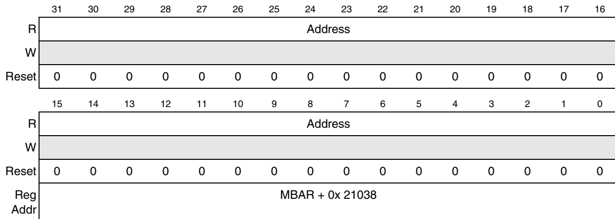
Figure 21-15. Master Error Address Register (MEAR)
