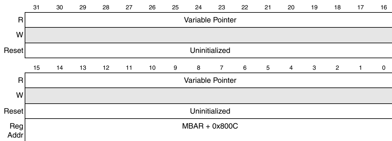
Figure 23-6. Variable Pointer Register (VP)
