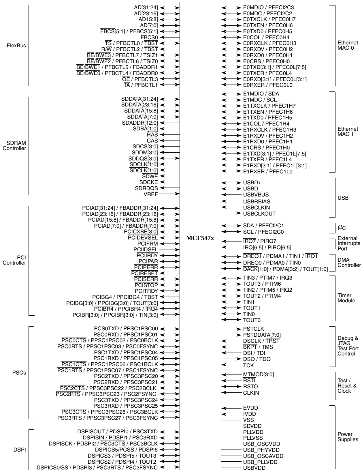
Figure 2-1. MCF547x Signals
