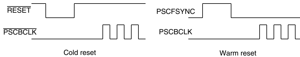
Figure 26-34. AC97 Cold and Warm Reset
