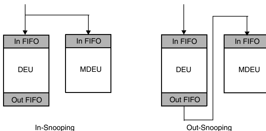
Figure 21-50. Snooping Example
