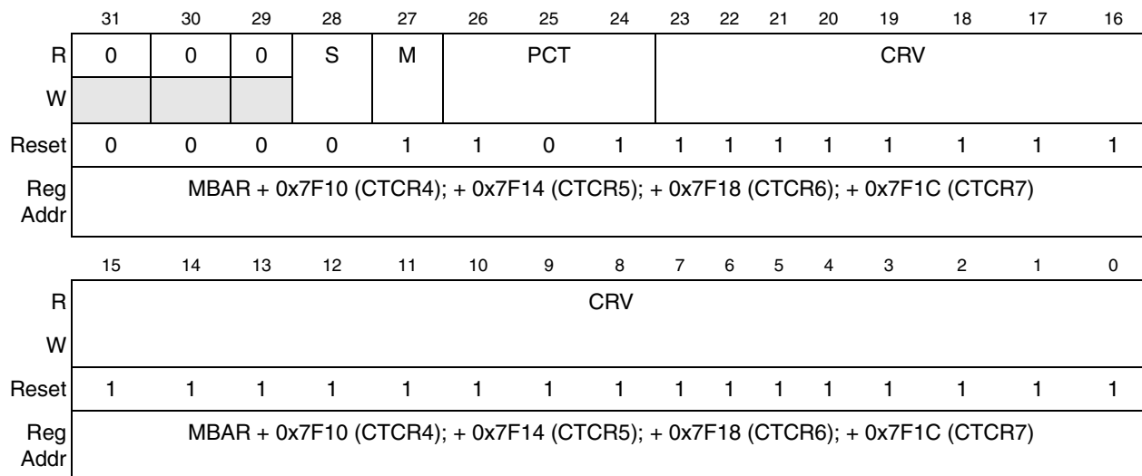
Figure 25-5. Comm Timer Configuration Register (CTCR4-CTCR7) —Variable Timer Channels
