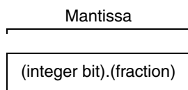
Figure 3-14. Mantissa
