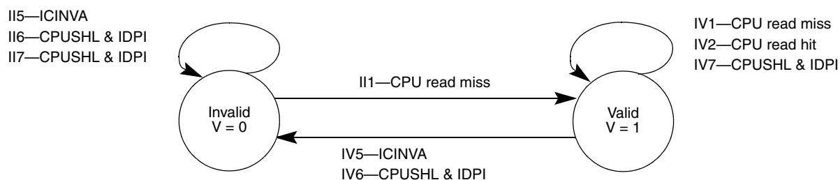
Figure 7-12. Instruction Cache Line State Diagram
