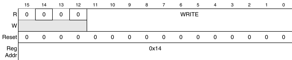
Figure 24-7. Write Pointer Register
