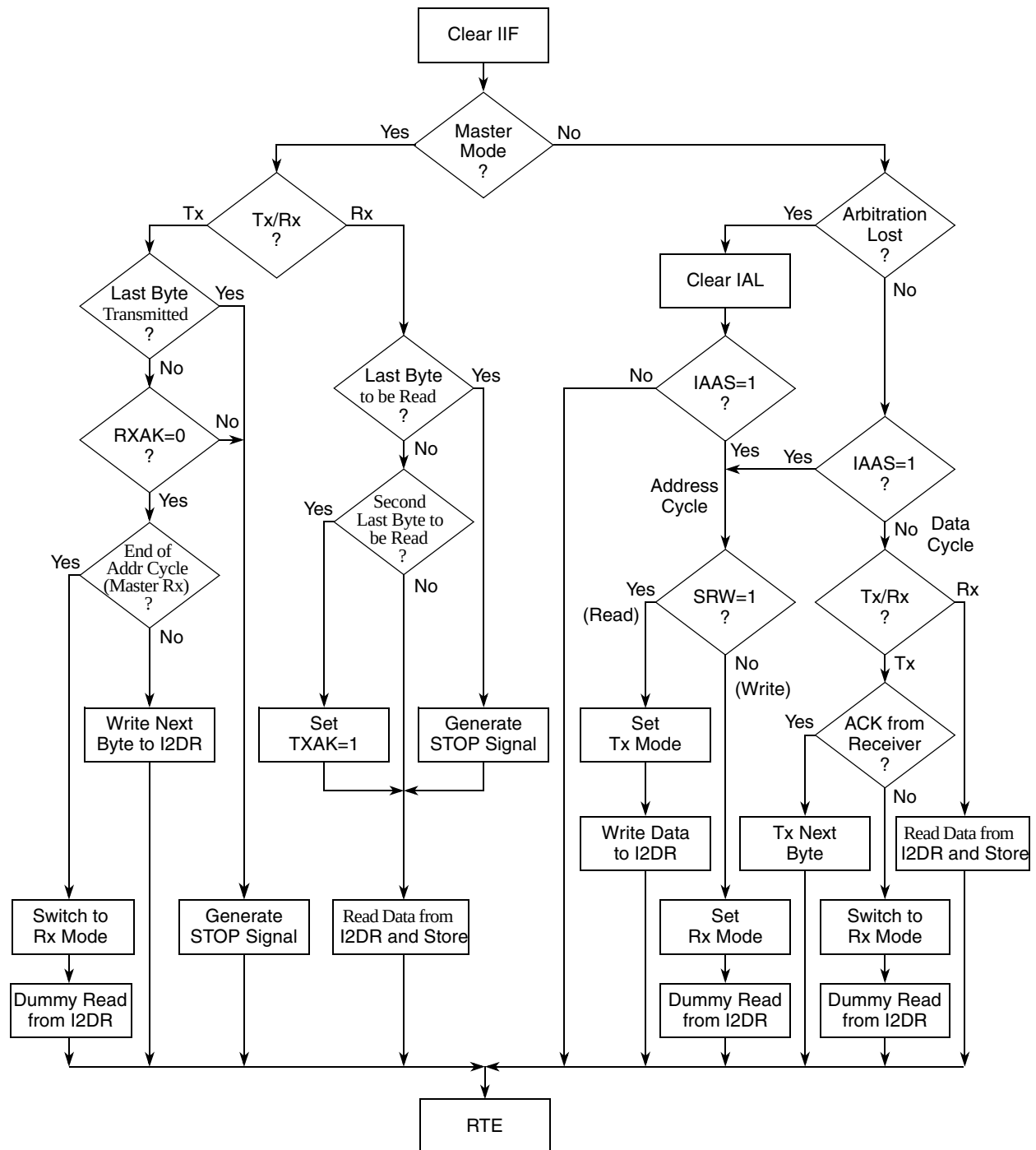
Figure 28-14. Flow-Chart of Typical I²C Interrupt Routine
