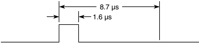
Figure 26-38. Serial Interaction Pulse (SIP)
