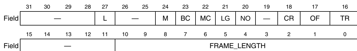
Figure 30-39. Receive Frame Status Word Format (RFSW)
