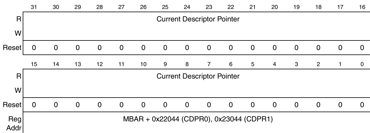
Figure 21-19. Crypto-Channel Current Descriptor Pointer Register (CDPR n )
