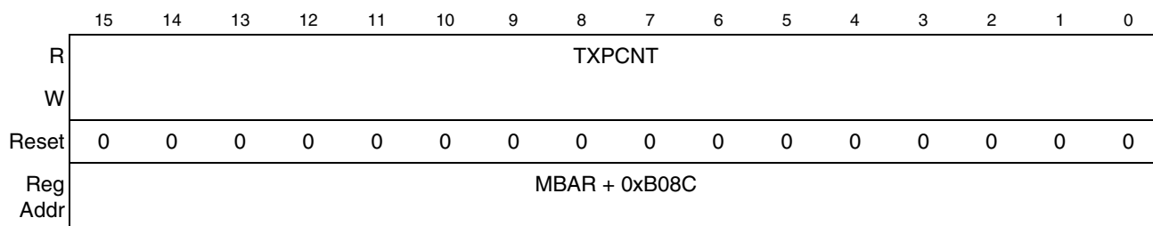
Figure 29-24. USB Transmitted Packet Counter Register (TXPCNT)
