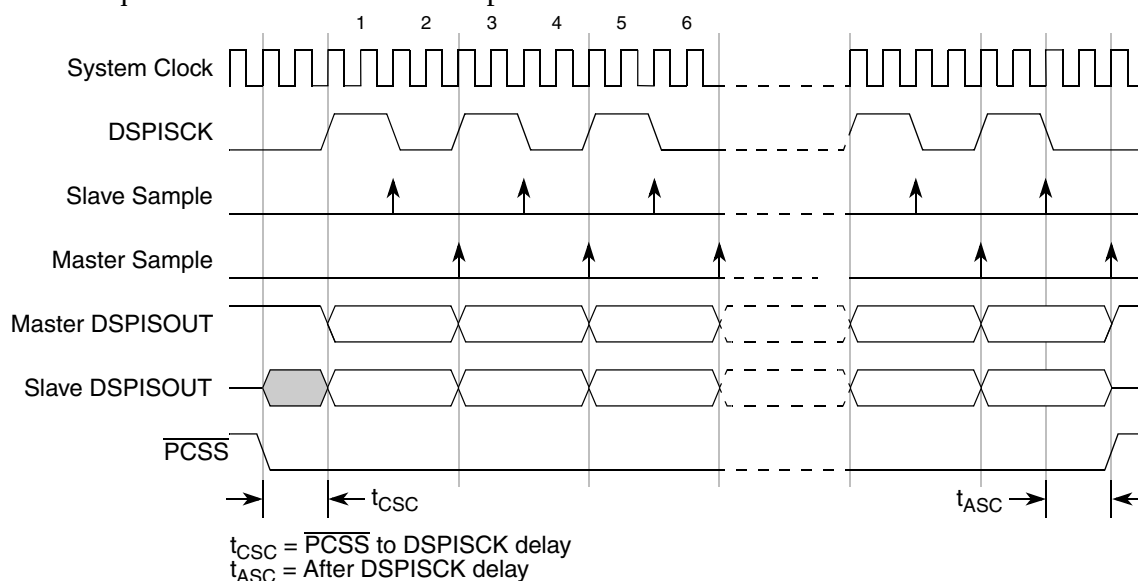
Figure 27-18. DSPI Modified Transfer Format (MTFE = 1, CPHA = 1, Fscck = Fsys/4)
