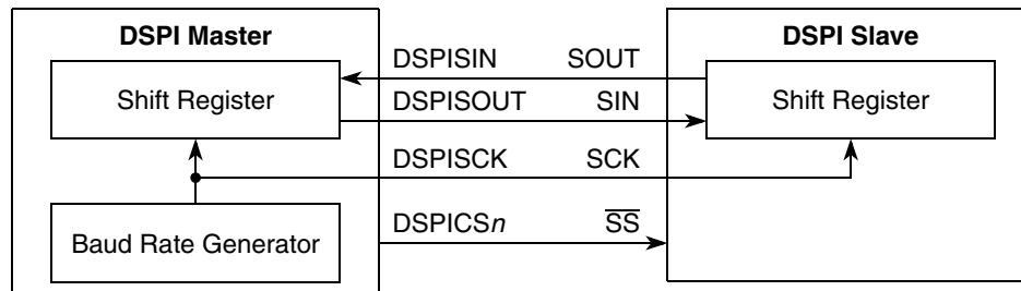
Figure 27-11. SPI Serial Protocol Overview
