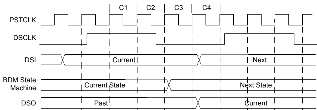
Figure 30-12. BDM Serial Interface Timing
