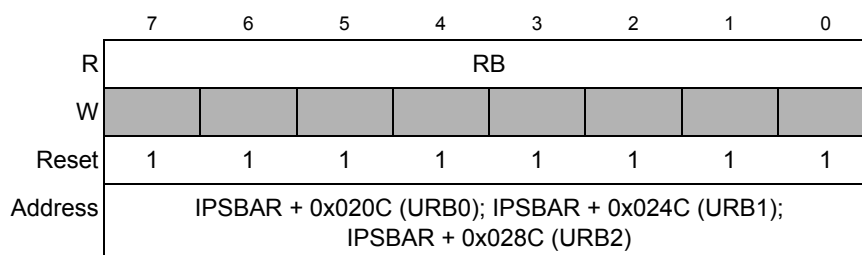
Figure 24-8. UART Receive Buffer (URB n )
