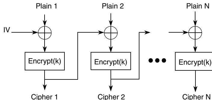
Figure 28-5. CBC Encryption
