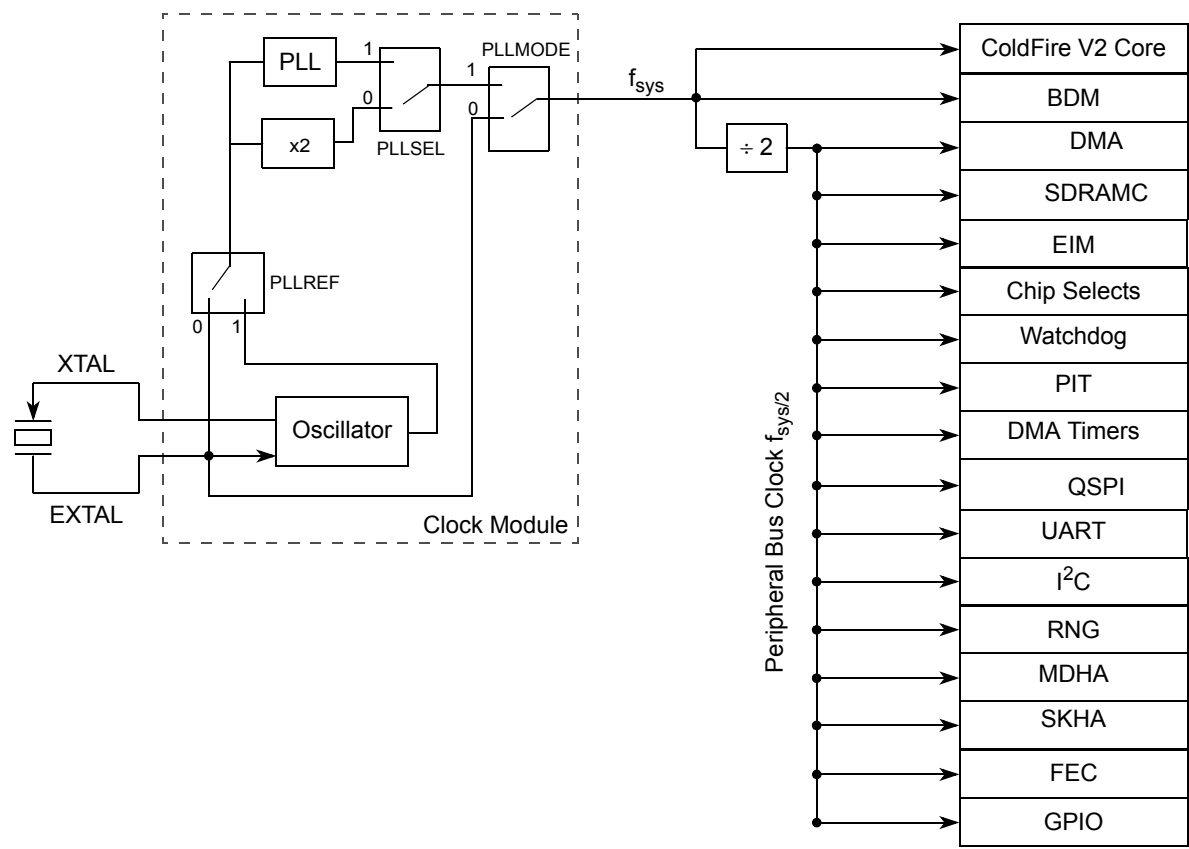
Figure 7-1. MCF5271 Clock Connections
