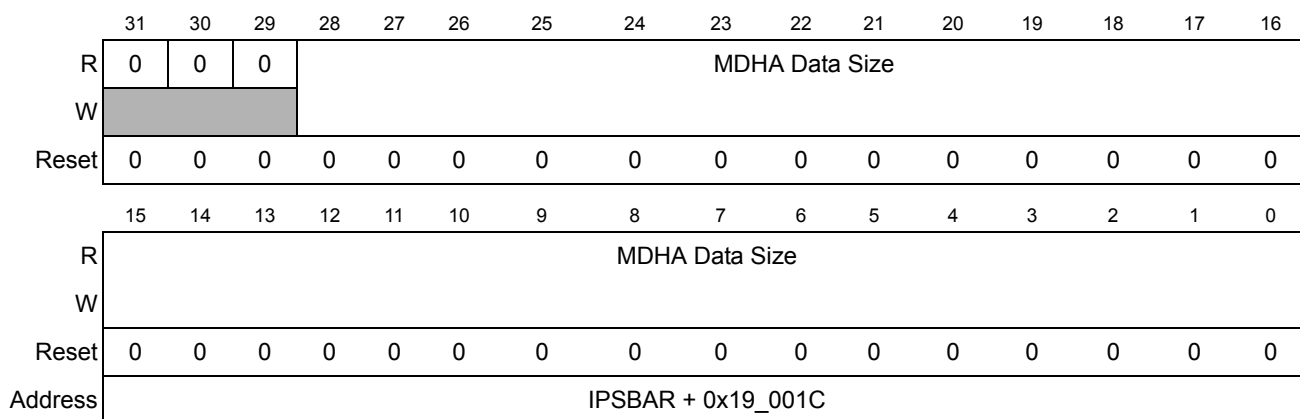
Figure 26-7. MDHA Data Size Register (MDDSR)
