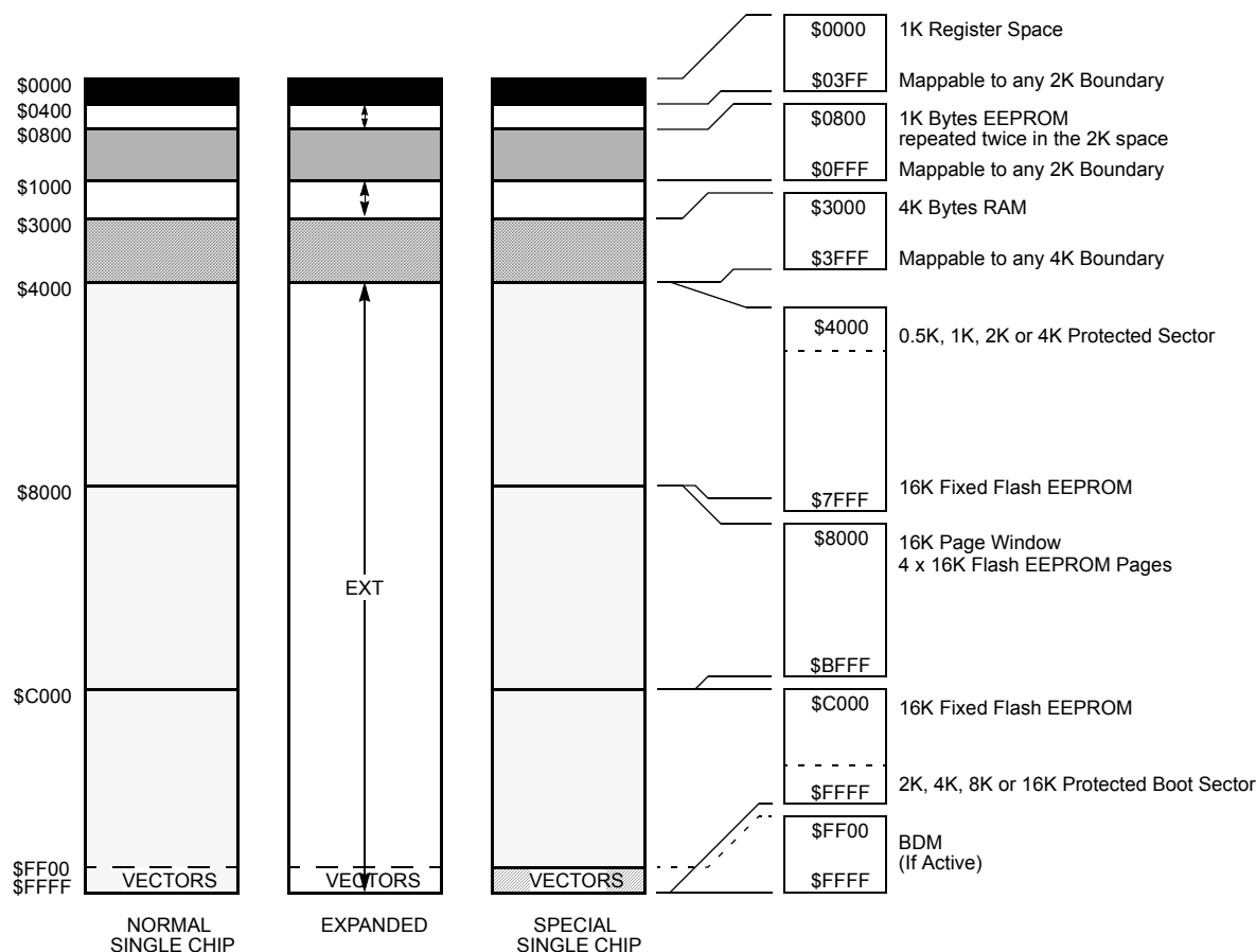
Figure 5 MC9S12K64 User Configurable Memory Map
