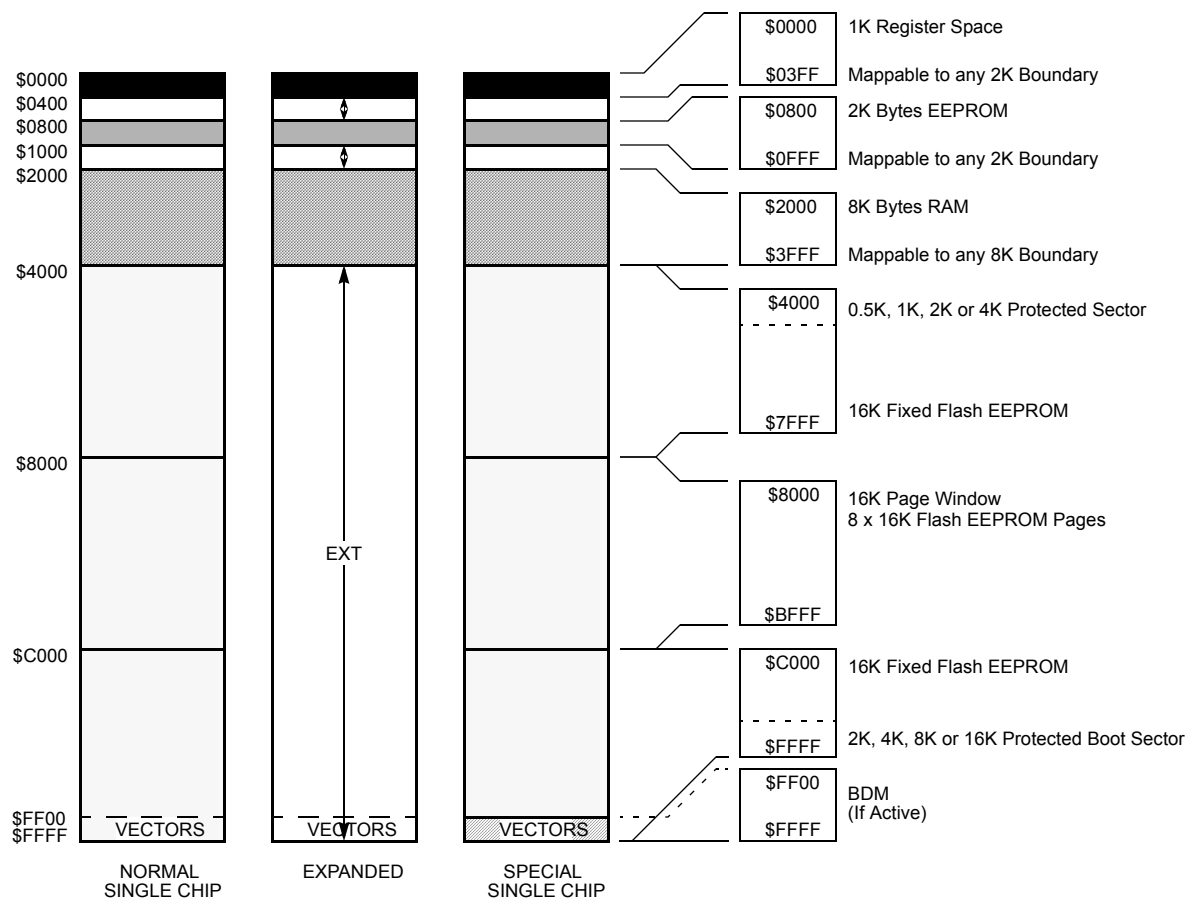
Figure 4 MC9S12KG128 User Configurable Memory Map
