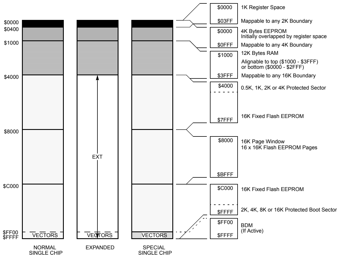
Figure 3 MC9S12Kx256 User Configurable Memory Map
