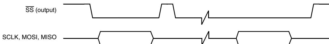
Figure 16. Master CSPI Timing Diagram Ignore \overline{\text{SPI\_RDY}} Level Trigger
