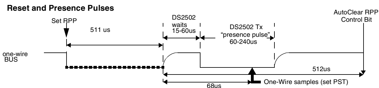
Figure 38. 1-Wire Initialization
