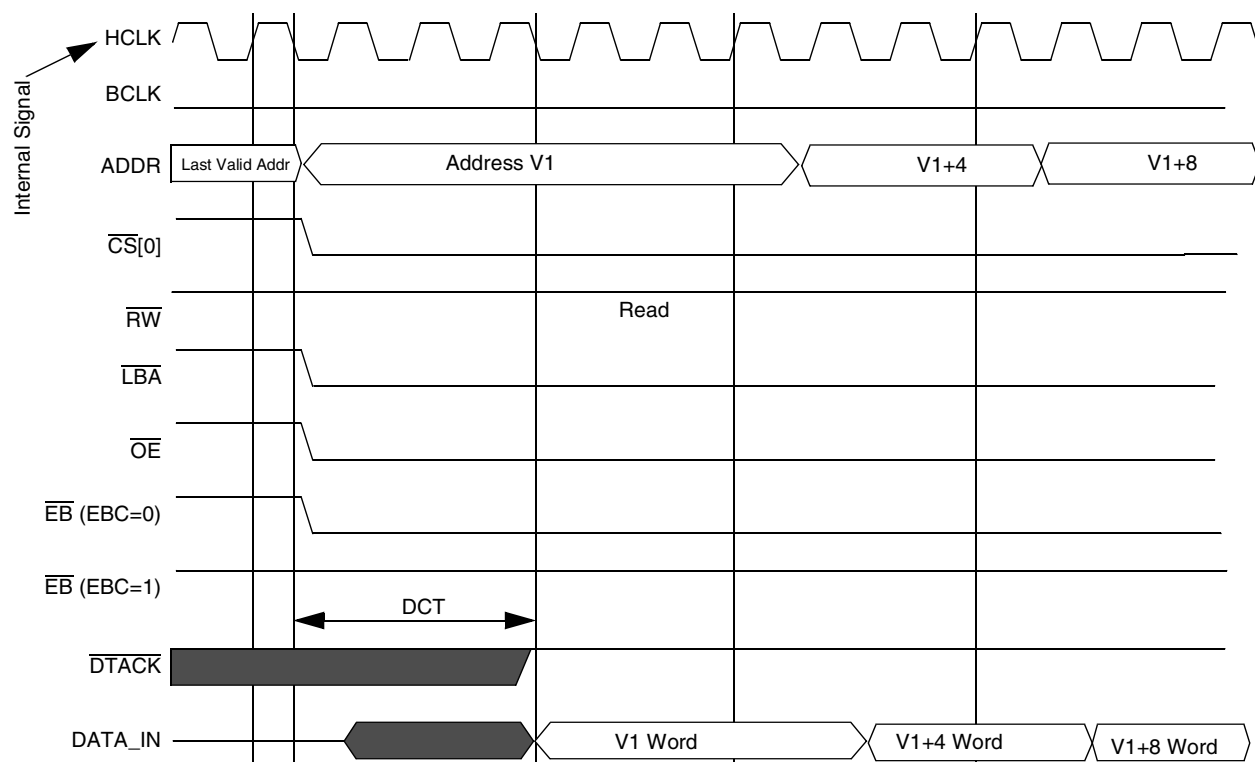
Figure 70. DTACK Level Sensitive Sequential Read Accesses, WSC=2, EW=1, DCT=1, AGE=0 (Example of \overline{DTACK} Remaining High)
