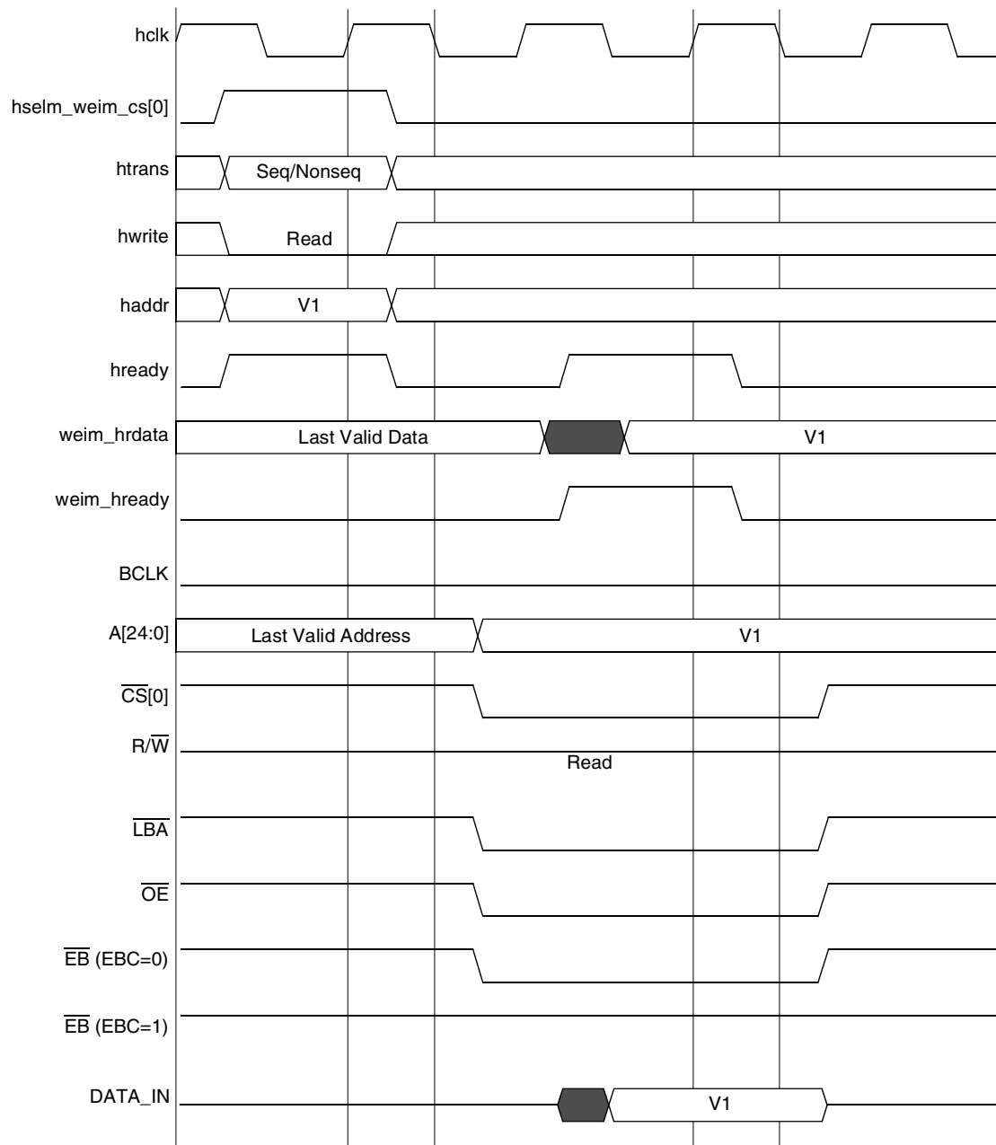
Figure 46. WSC = 1, A.HALF/E.HALF
