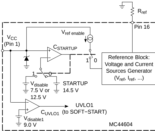
Figure 38. V_{CC} Management
