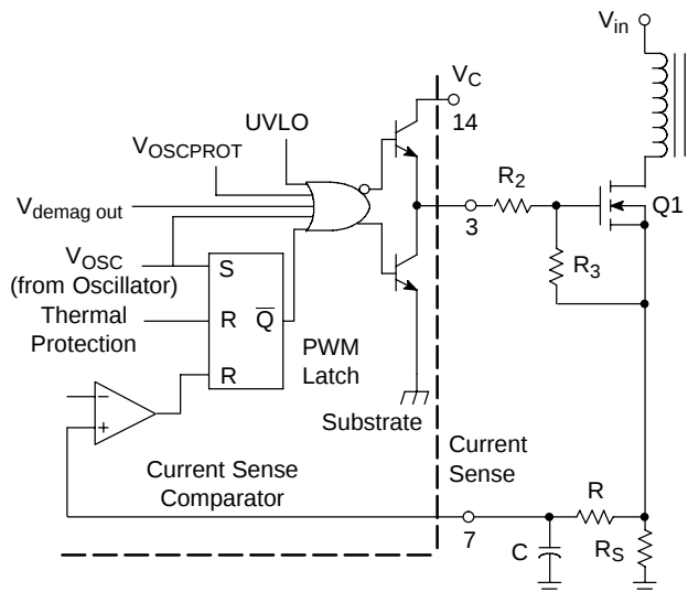
Figure 29. Output Totem Pole
