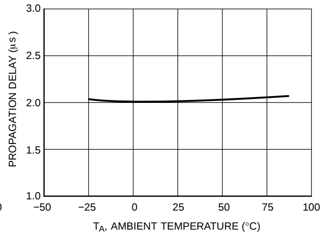
Figure 4. Propagation Delay Current (V otp > 2.58 V to V otp Low) vs. Temperature
