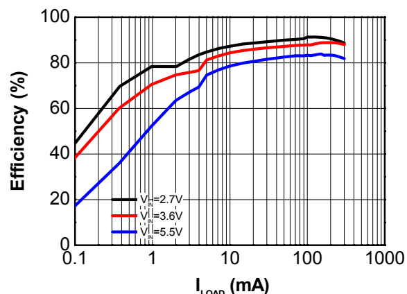
Figure 4. Efficiency vs. Load Current V_{IN} = 3.6V , V_{OUT} = 1.8V , T_A = 25^\circ C
