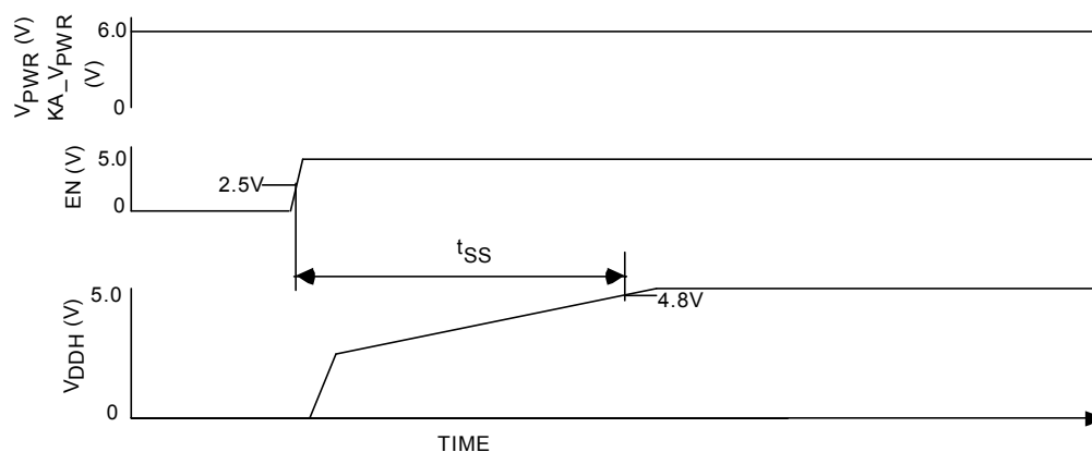
Figure 2. Soft-Start Time
