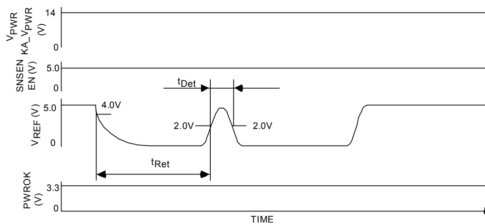
Figure 3. VREF Retry Timer
