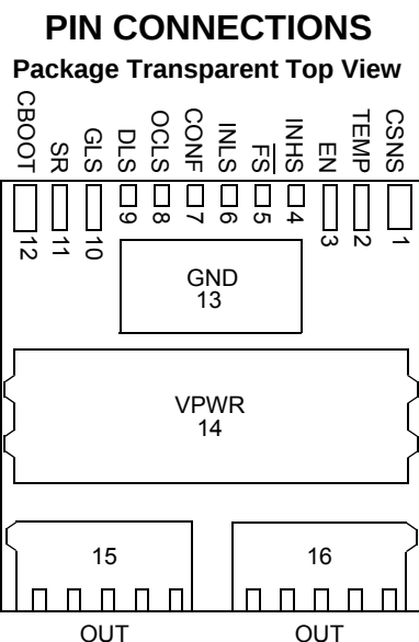
Figure 3. Pin Connections
