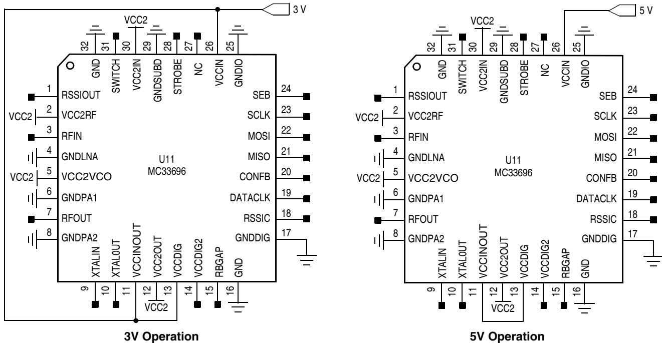
Figure 2. Wiring Diagrams
