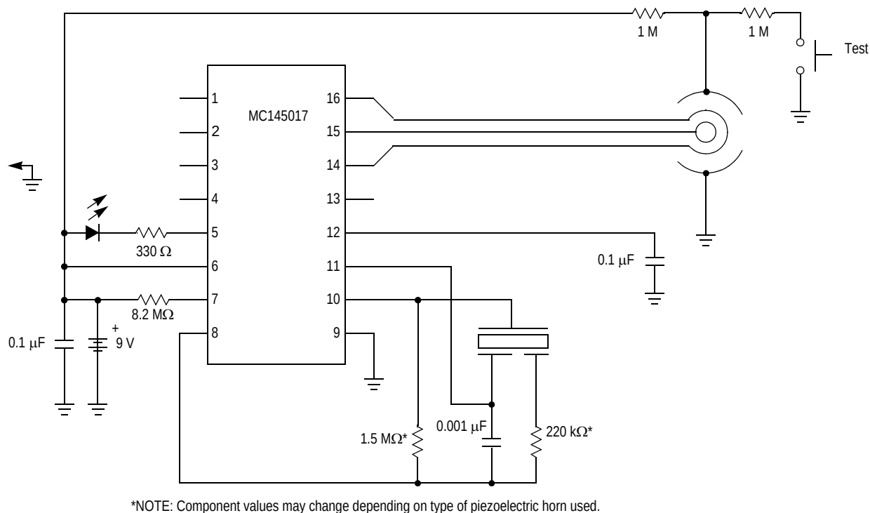
Figure 6. Typical Application as Ionization Smoke Detector
