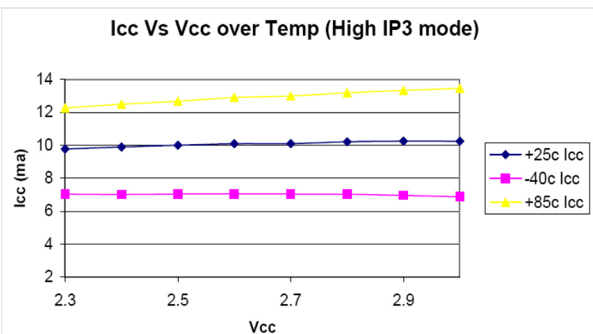
Figure 5. Icc vs Vcc Over Temperature (High IP3 Mode)
