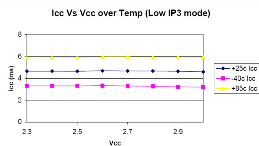
Figure 4. Icc vs Vcc Over Temperature (Low IP3 Mode)
