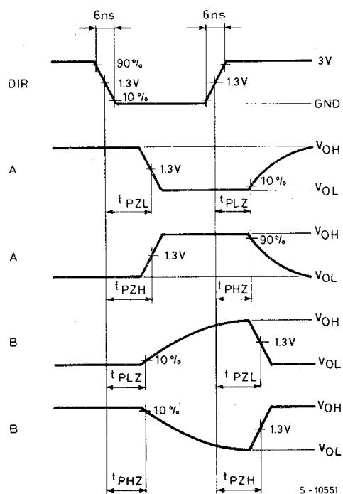
WAVEFORM 4 : OUTPUT ENABLE AND DISABLE TIME (f=1MHz; 50% duty cycle)
