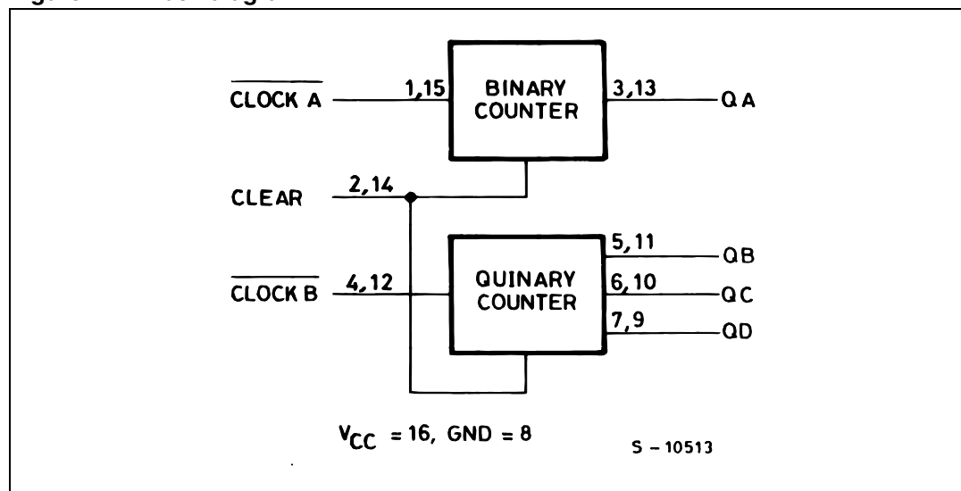
Figure 5. Logic diagram
