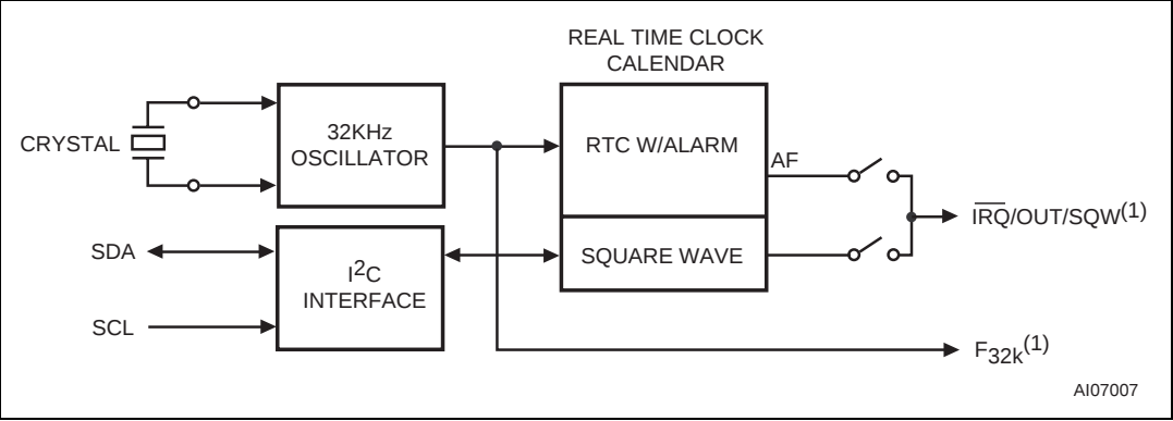
Figure 3. Block diagram
