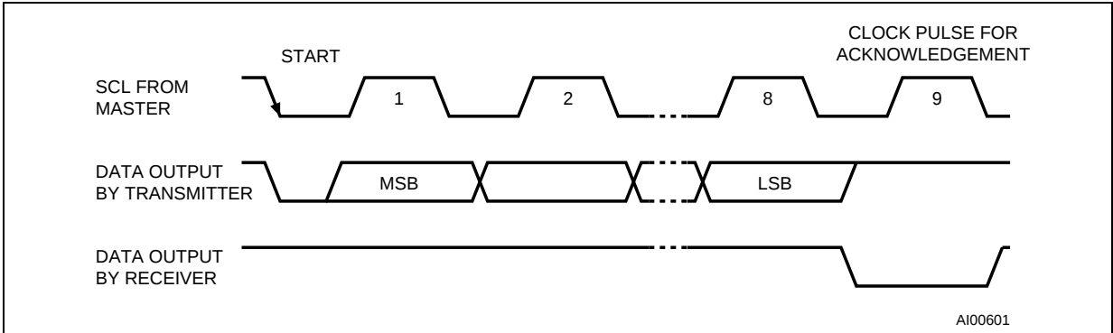
Figure 5. Acknowledgement sequence
