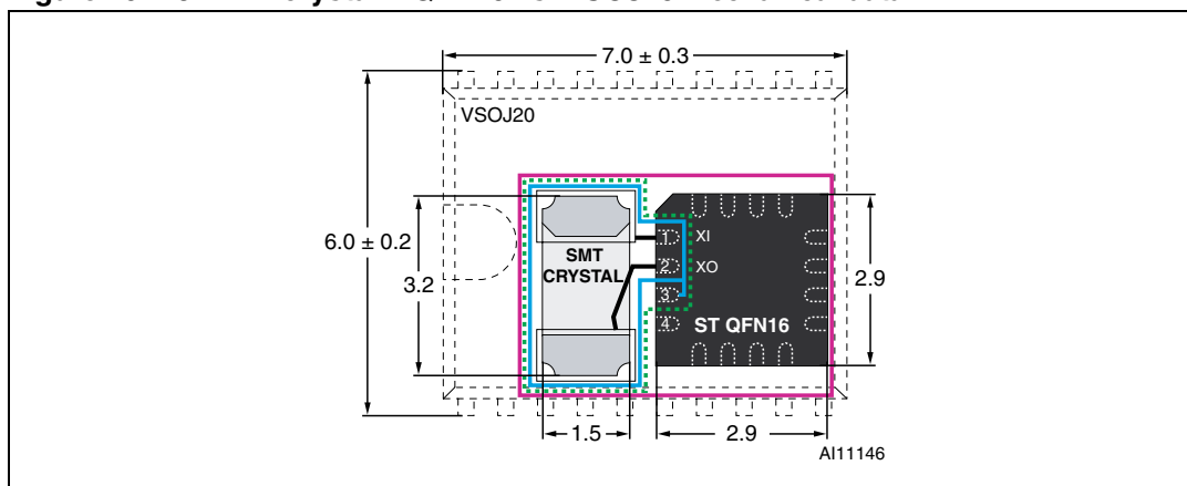
Figure 19. 32 KHz crystal + QFN16 vs. VSOJ20 mechanical data
