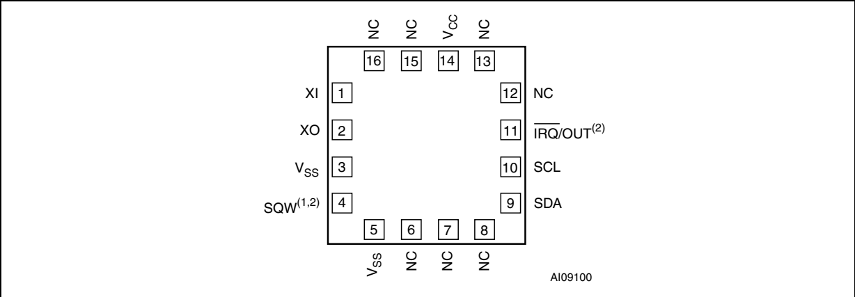
Figure 2. M41T66 connections
