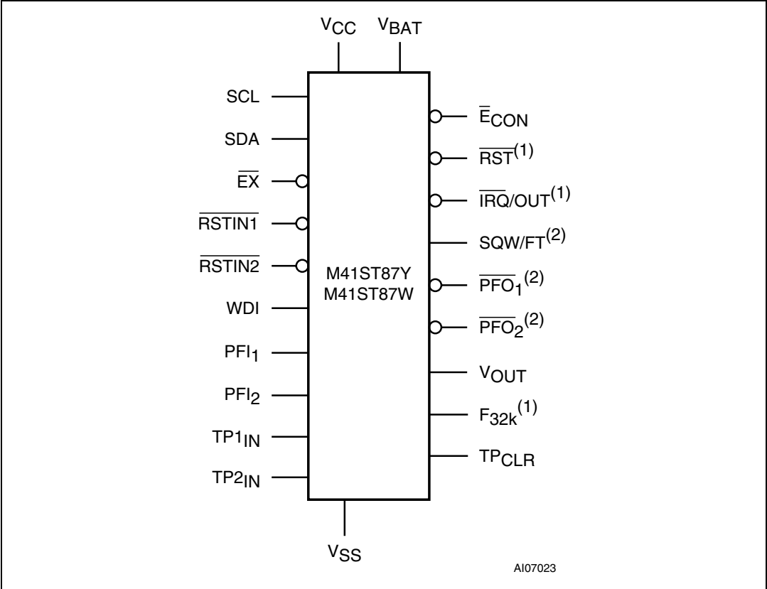
Figure 1. Logic diagram
