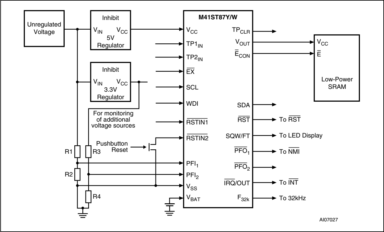
Figure 4. Hardware hookup
