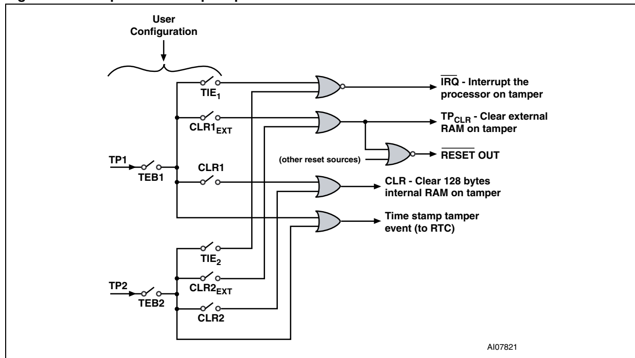
Figure 14. Tamper detect output options
