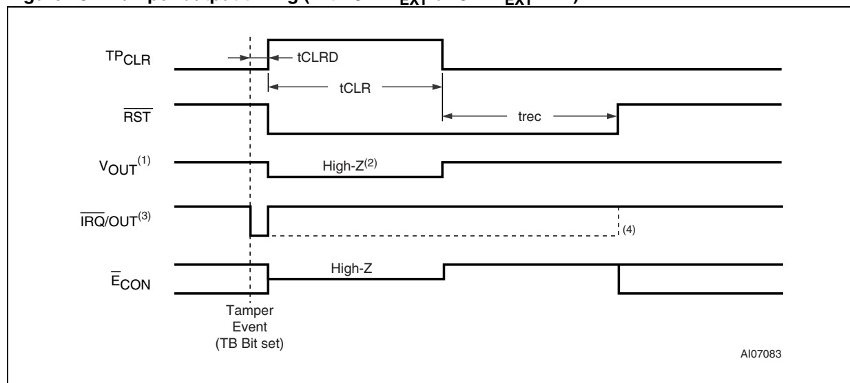
Figure 18. Tamper output timing (with CLR1 EXT or CLR2 EXT = '1')
