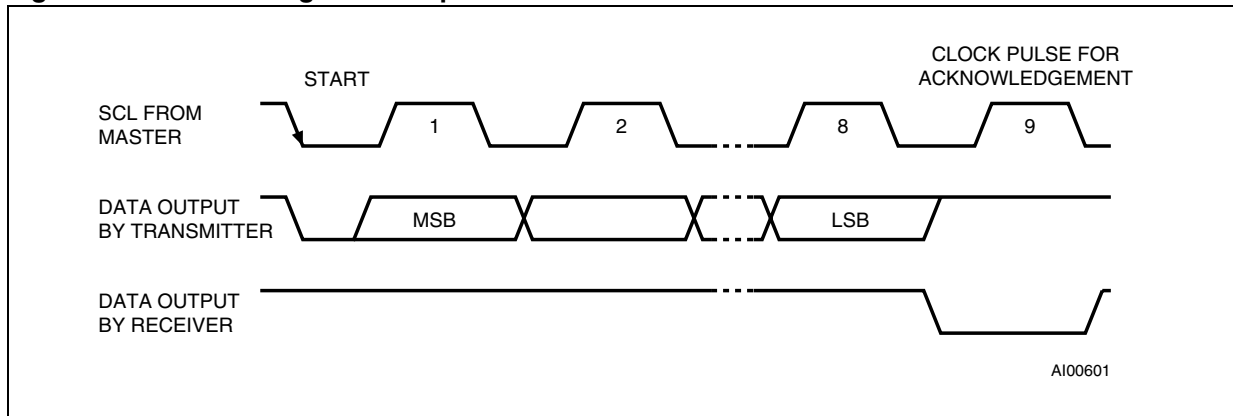
Figure 6. Acknowledgement sequence
