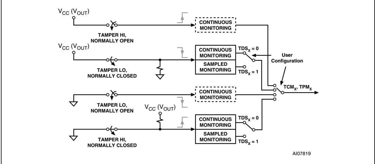
Figure 16. Tamper detect sampling options
