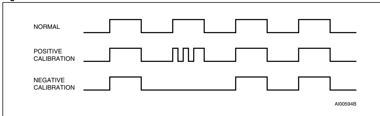
Figure 22. Calibration waveform
