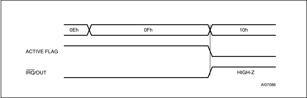
Figure 23. Alarm interrupt reset waveform
