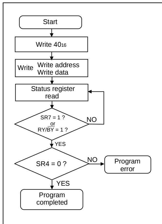
Fig. 119 Program flowchart
