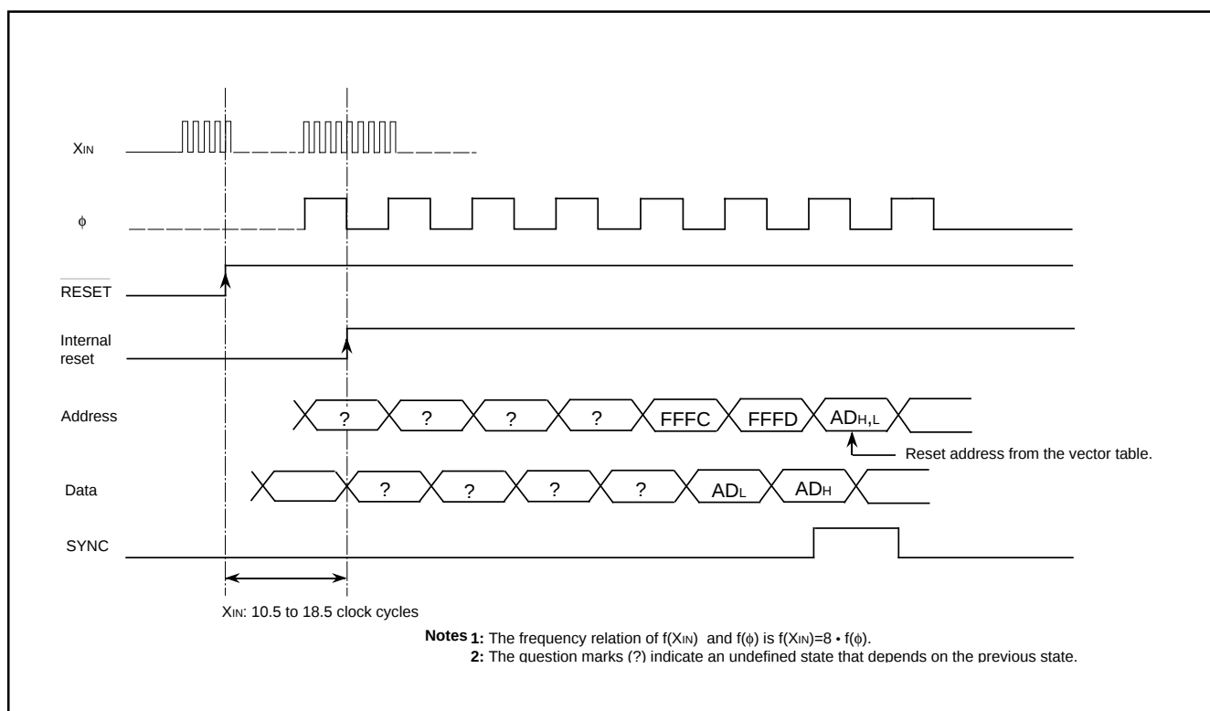
Fig. 79 Reset sequence
