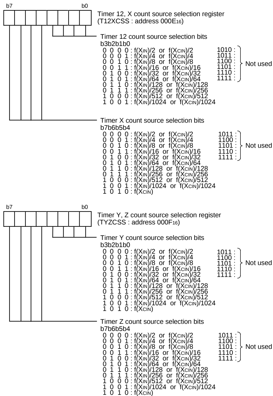
Fig. 31 Structure of timer 12, X and timer Y, Z count source selection registers
