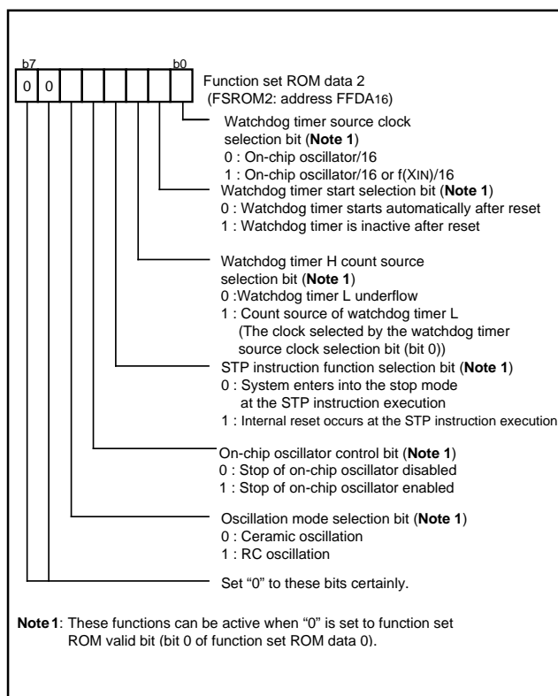
Fig. 85 Structure of Function set ROM data 2
