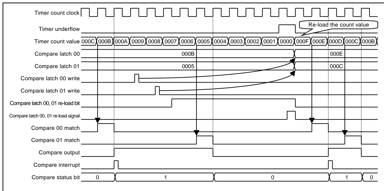
Fig. 40 Output compare mode (compare register write timing)
