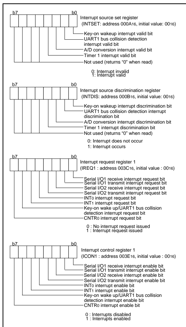
Fig. 54 Bus collision detection circuit related registers
