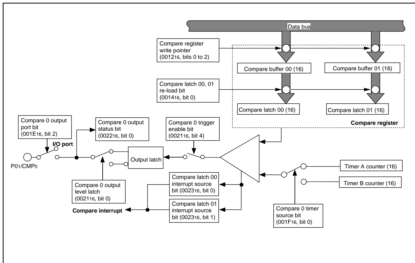
Fig. 37 Block diagram of compare channel 0
