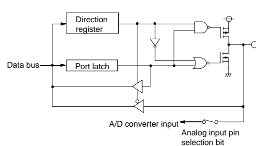
(13) Ports P20–P25
