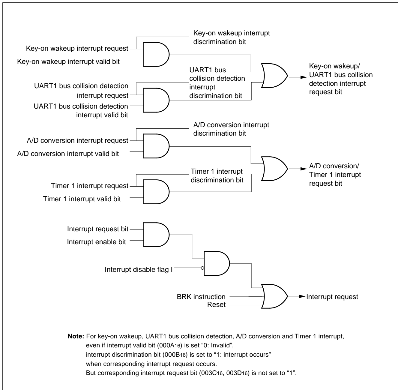
Fig. 20 Interrupt control
