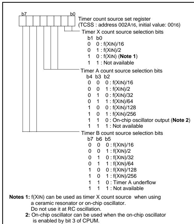
Fig. 27 Timer count source set register
