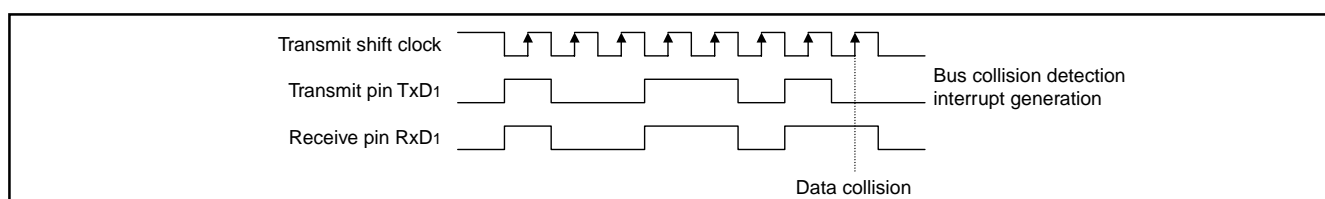
Fig. 56 Timing diagram of bus collision detection interrupt
