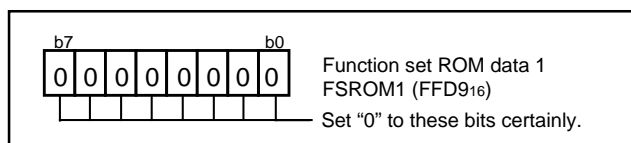
Fig. 84 Structure of Function set ROM data 1
