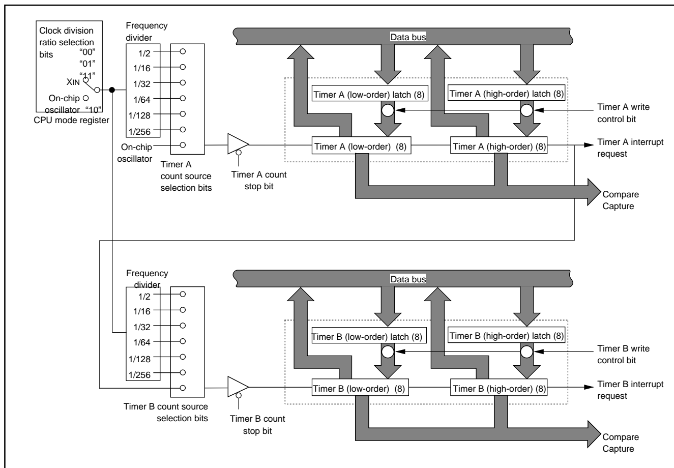
Fig. 28 Block diagram of timer A and timer B
