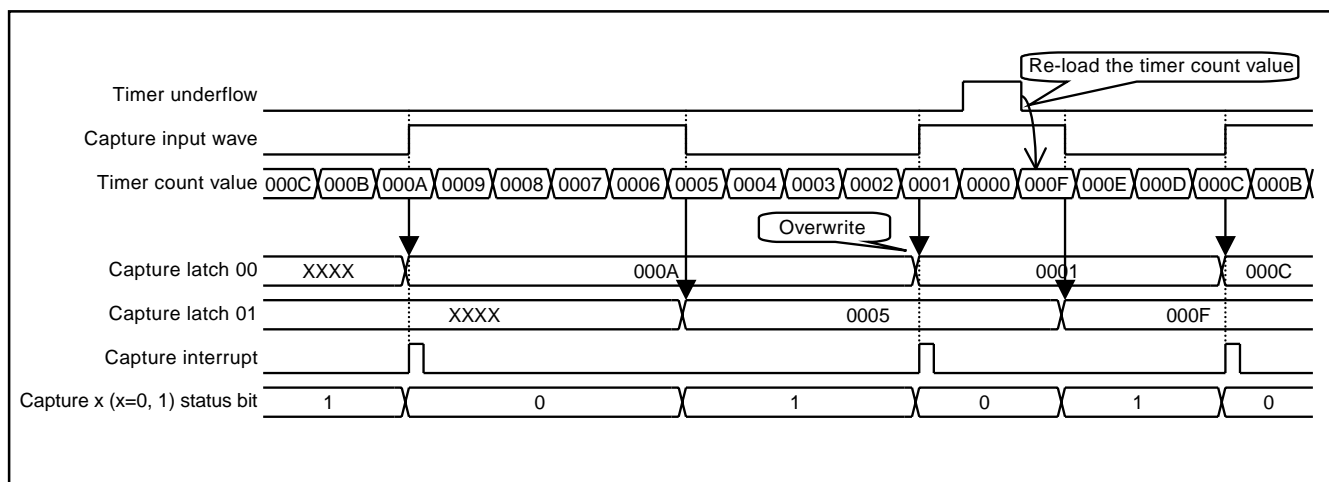
Fig. 47 Capture interrupt edge selection = "rising edge"
