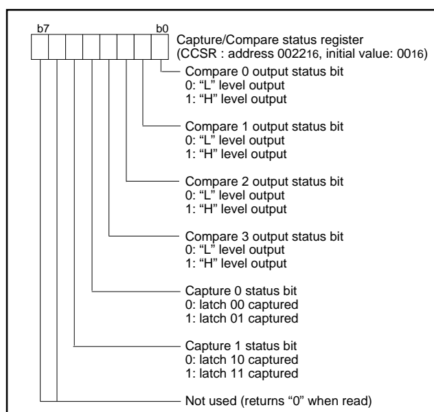
Fig. 34 Structure of capture/compare status register
