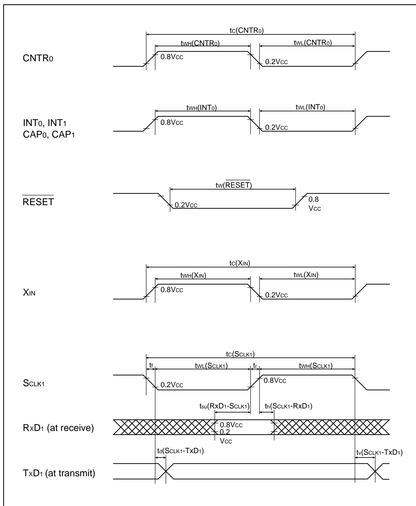
Fig. 95 Timing chart
