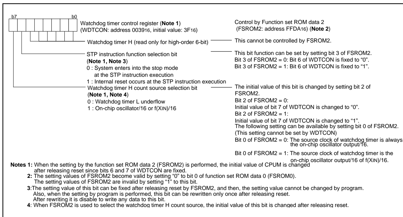
Fig. 66 Structure of watchdog timer control register
