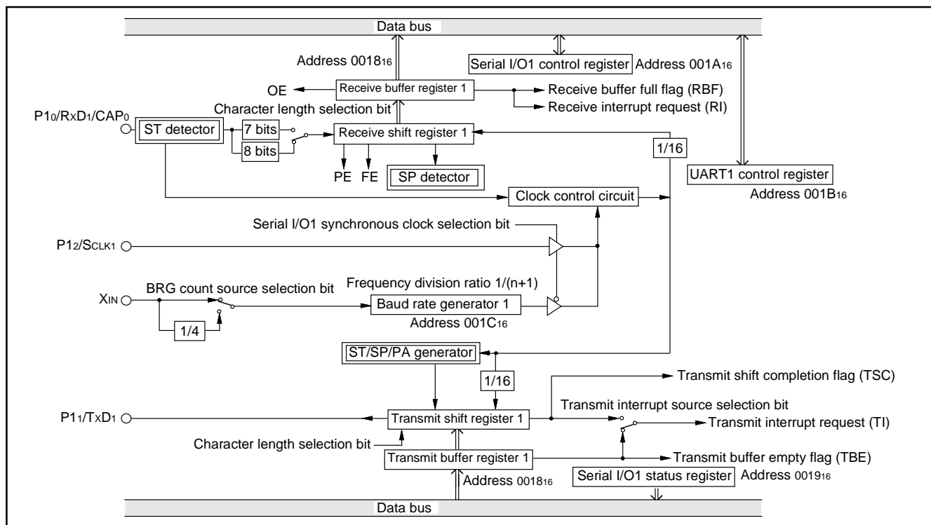
Fig. 51 Block diagram of UART serial I/O1
