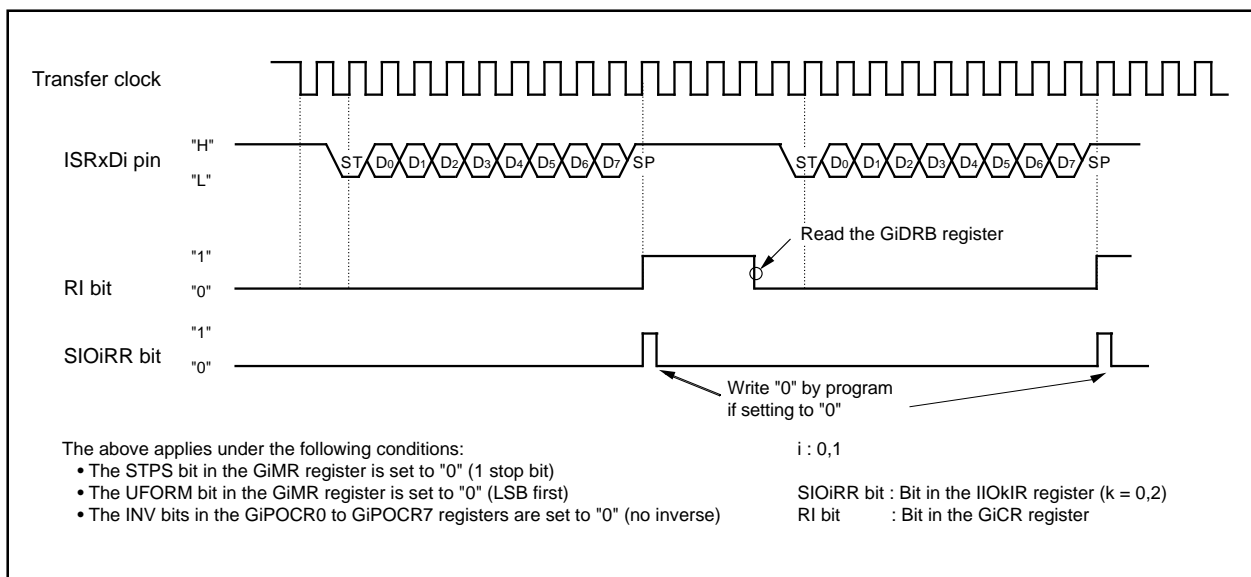
Figure 21.41 Receive Operation
