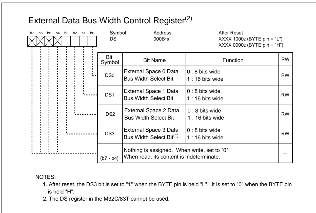
Figure 7.1 DS Register
