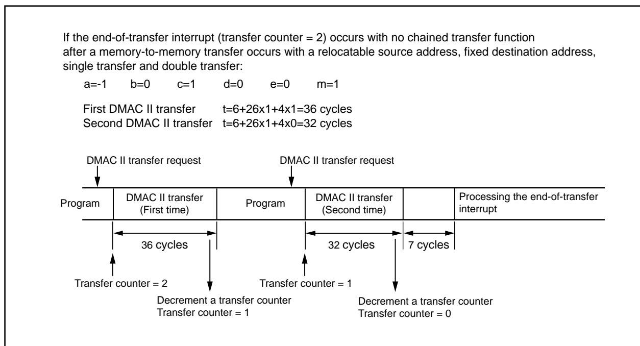
Figure 13.5 Transfer Cycle
