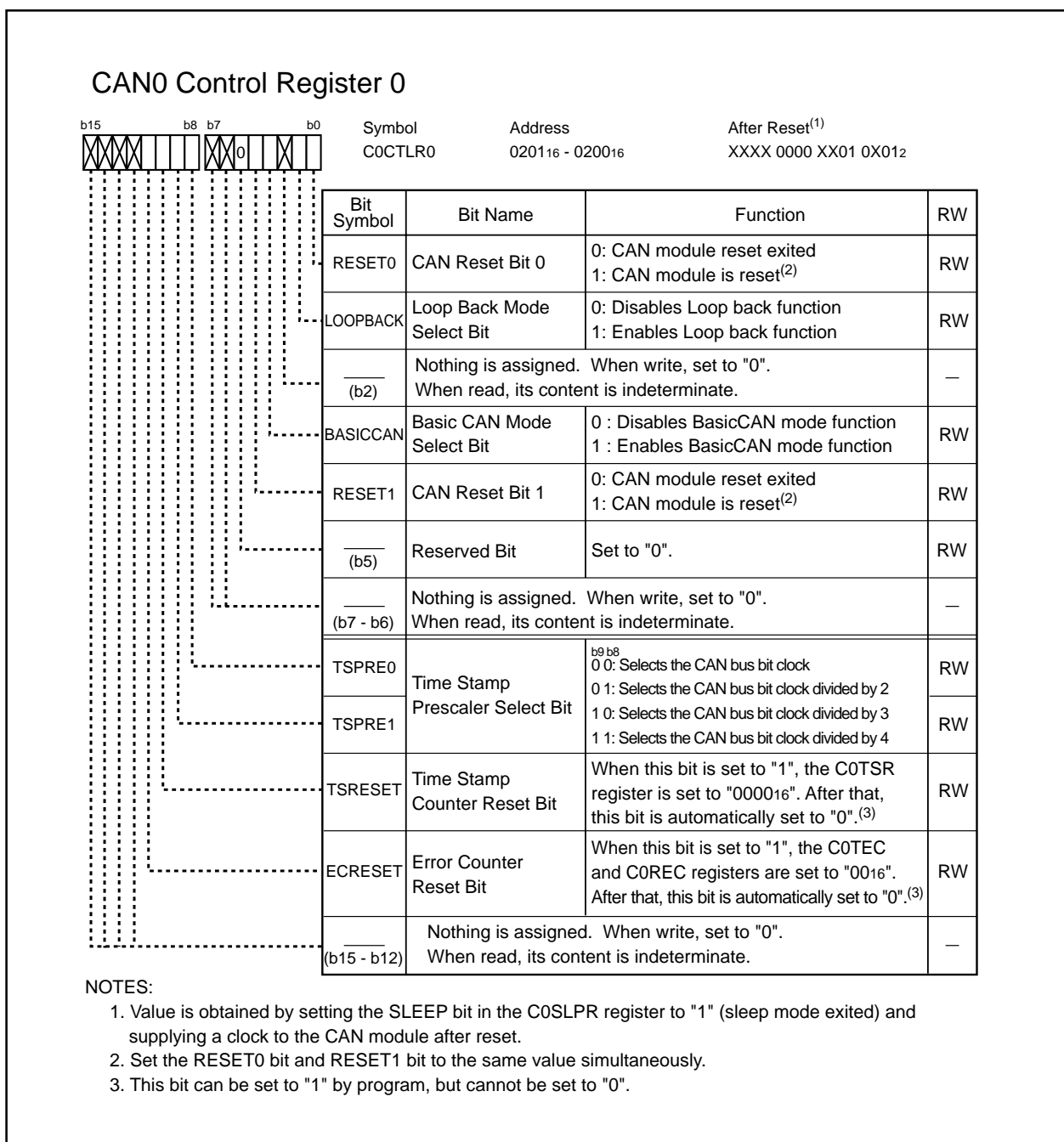
Figure 22.3 C0CTRL0 Register
