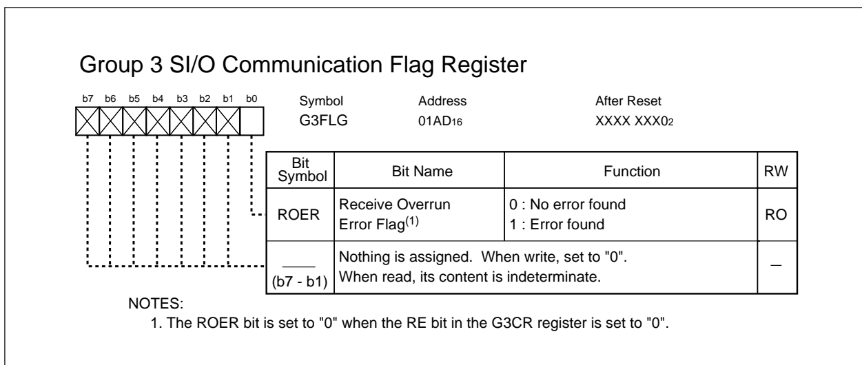
Figure 21.49 G3FLG Register
