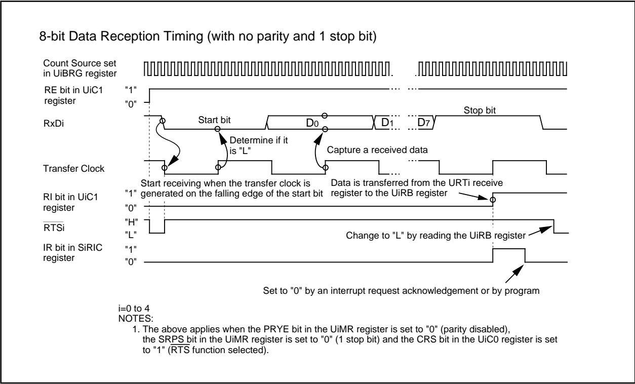
Figure 16.15 Receive Operation
