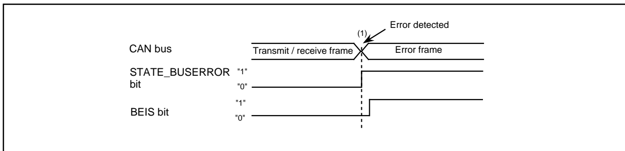
Figure 22.30 Operation Timing when CAN Bus Error Occurs
