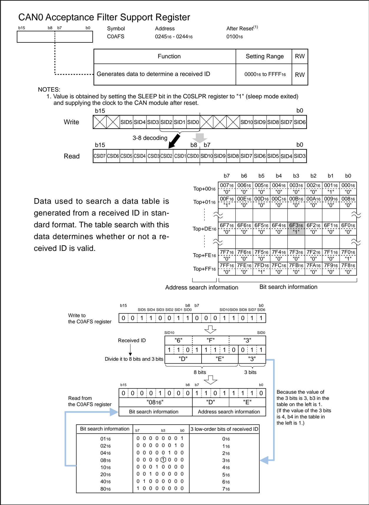
Figure 22.26 C0AFS Register
