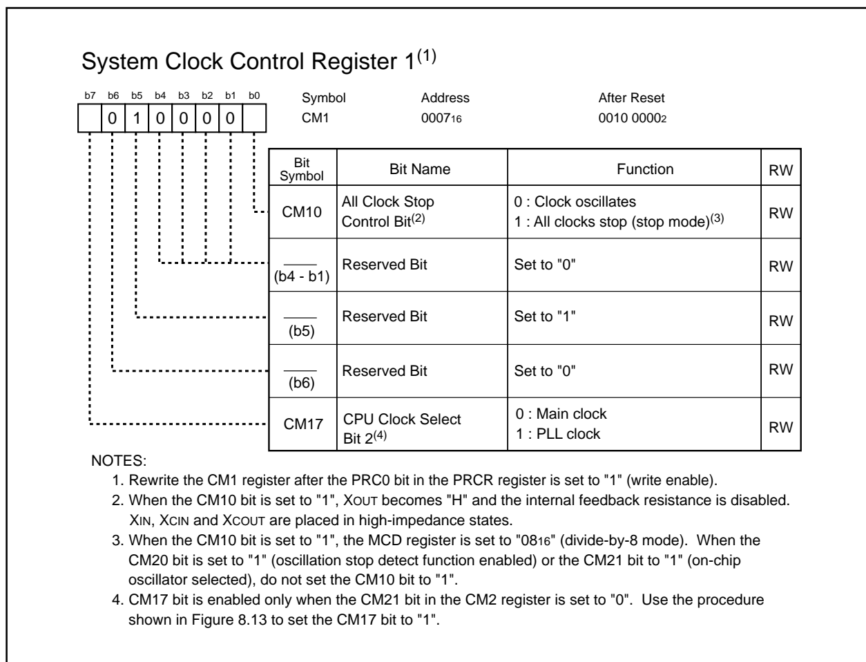
Figure 8.3 CM1 Register
