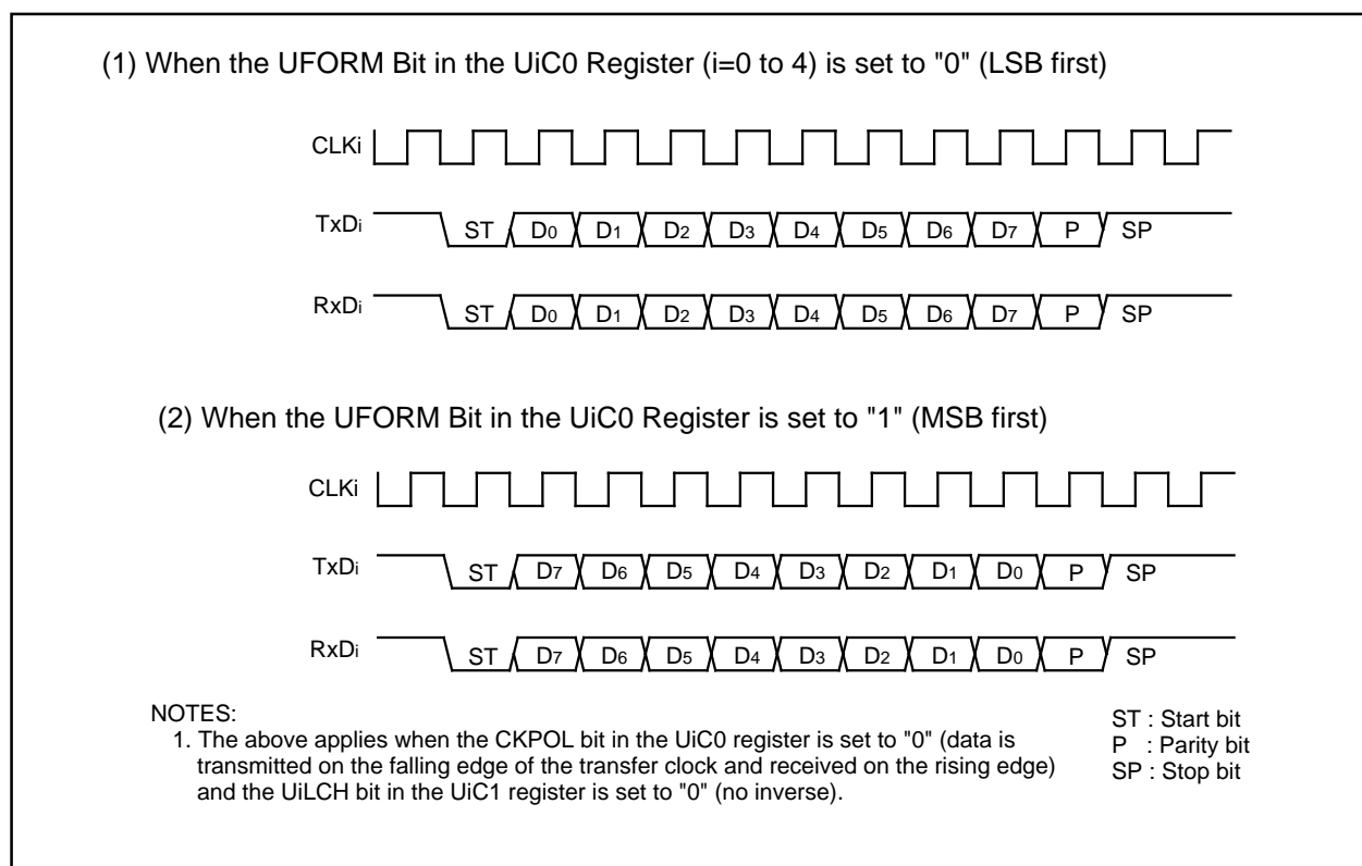
Figure 16.16 Transfer Format
