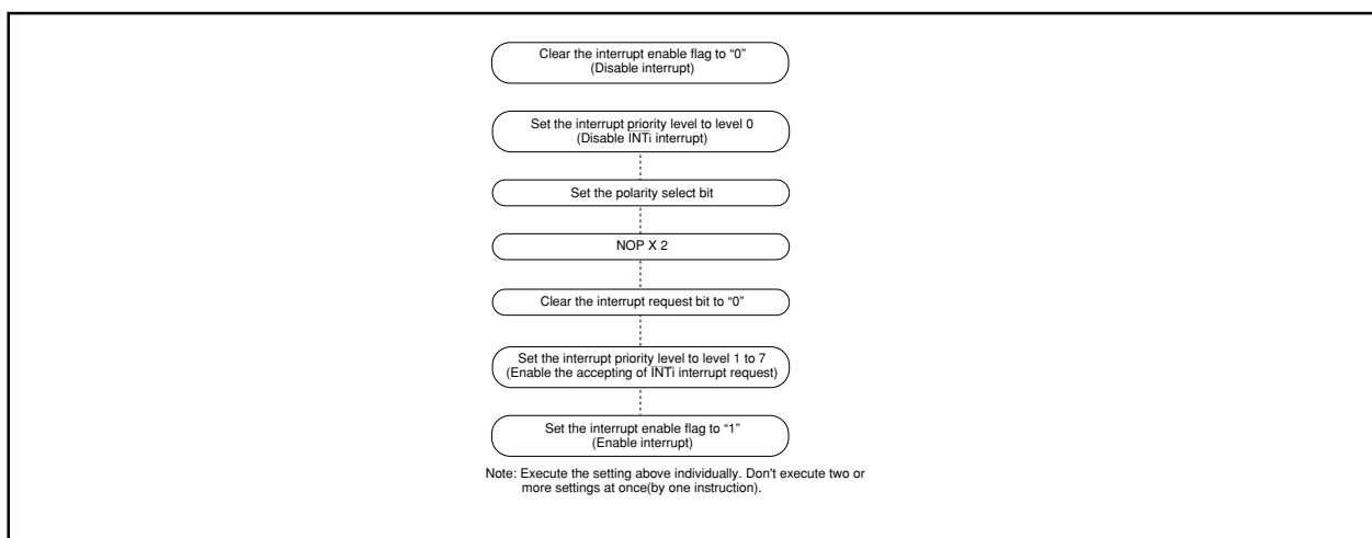
Figure 1.11.13. Switching condition of INT interrupt request
