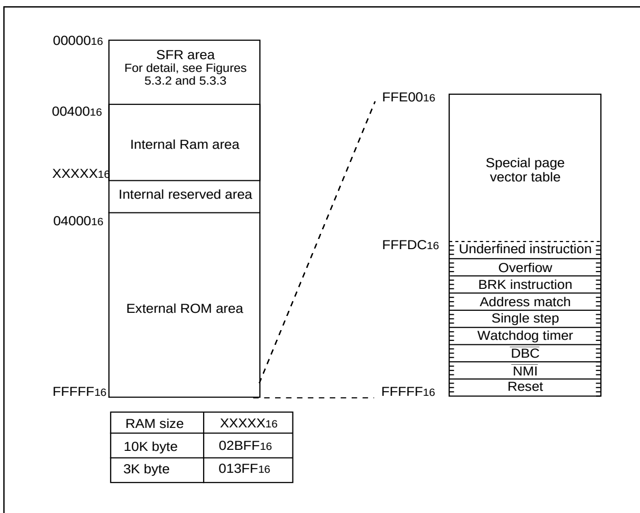
Figure 5.3.1. Memory map
