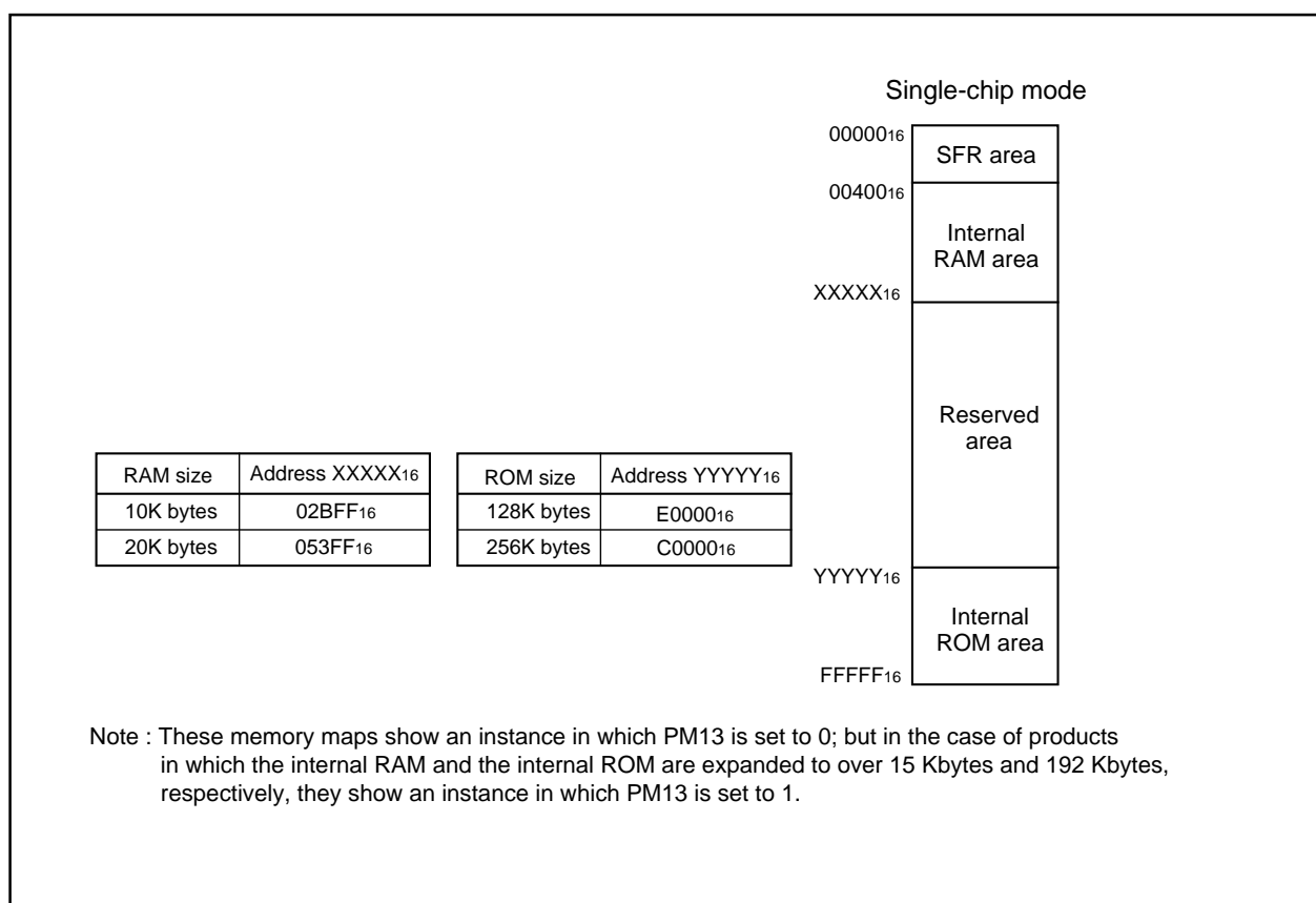
Figure 1.8.2. Memory map
