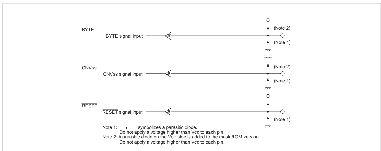
Figure 1.136. I/O pins
