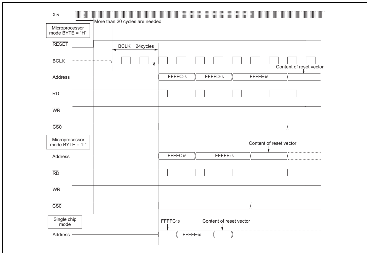
Figure 1.9. Reset sequence
