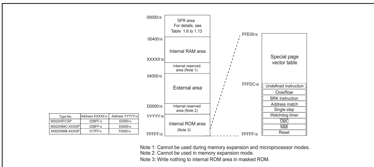
Figure 1.5. Memory map
