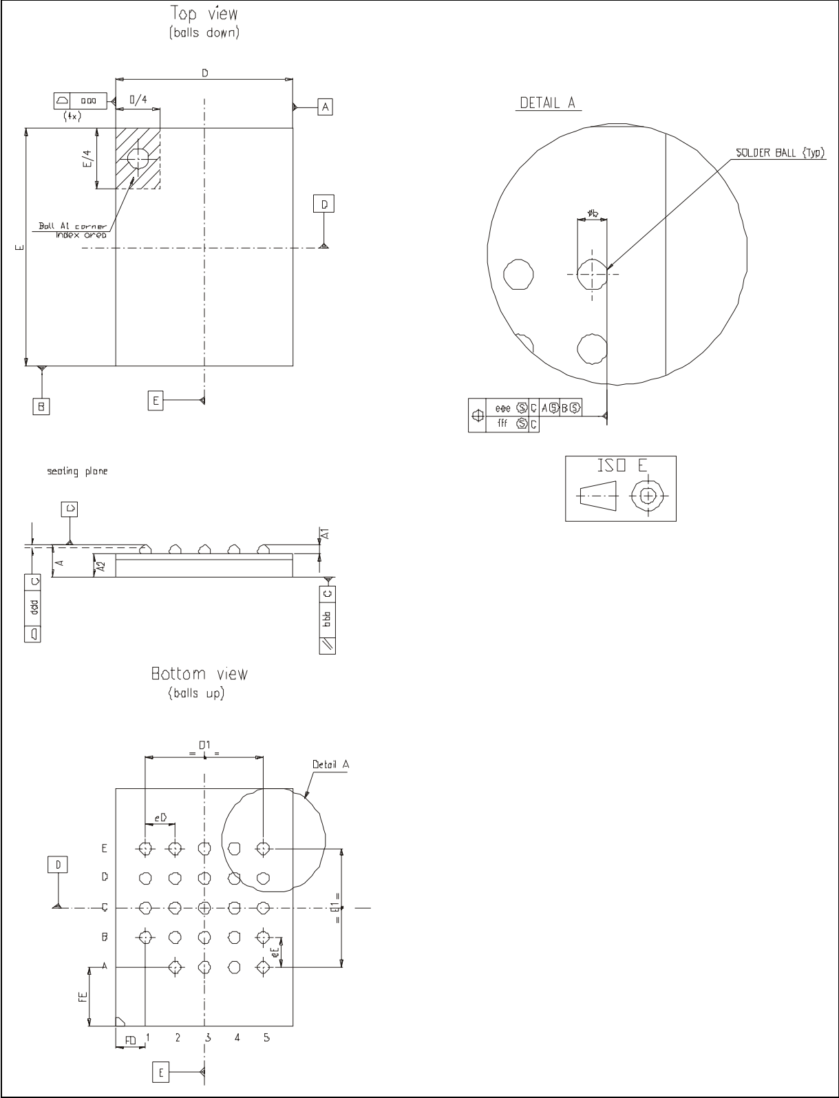
Figure 37. TBGA, 6x8 mm, 24 ball package outline
