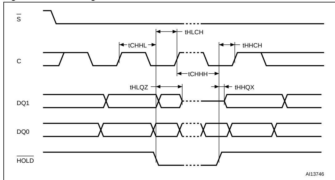
Figure 32. Hold timing
