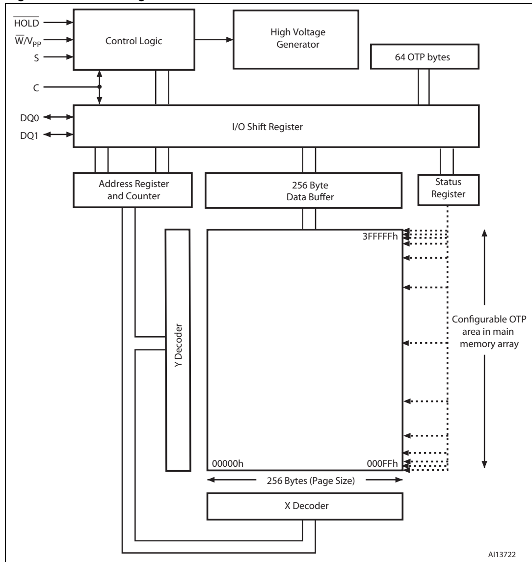
Figure 7. Block diagram
