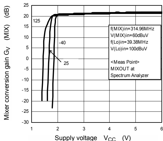
Mixer Conversion Gain – Supply Voltage Characteristics
