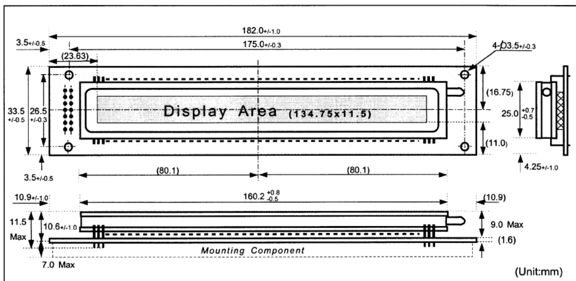
Fig-7 Outer dimensions
