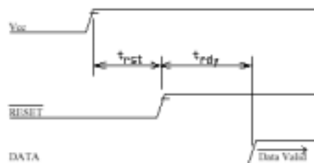
Figure 5. Power-up and Reset timing
