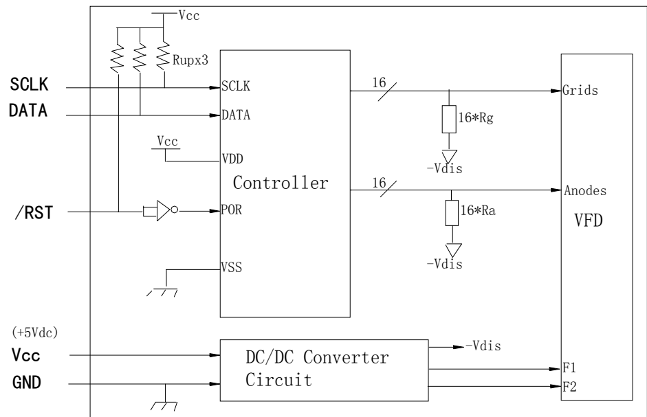
Fig-3 VFD Module System Block Diagram
