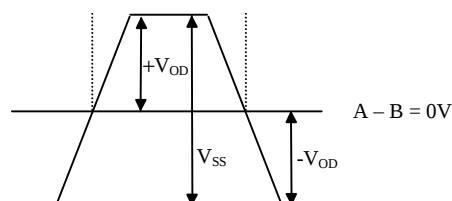
Figure 4: Single-ended & Differential Waveforms
