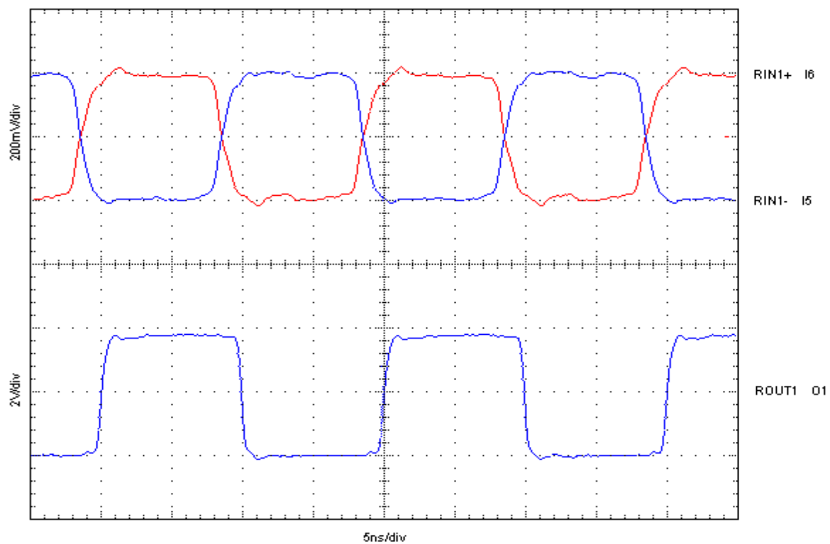
Figure 10: LVDS Cannel #1B Waveforms – A Small Amount of Common Mode Noise Coupled from Output to Input
