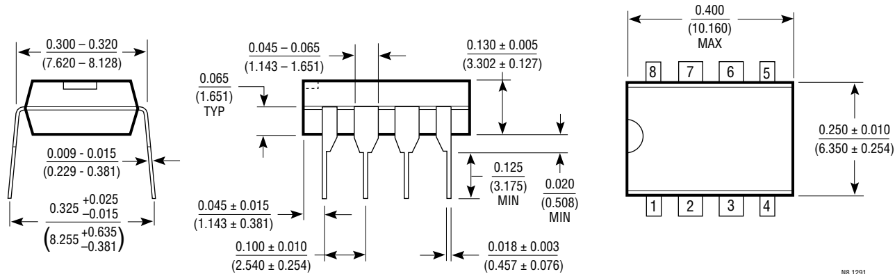
N8 Package 8-Lead Plastic DIP
