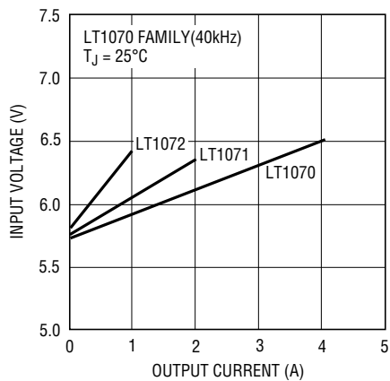
Minimum Input Voltage – Normal Mode (1070 Family)
