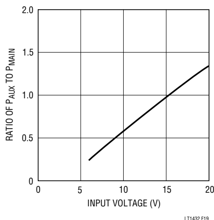
Figure 19. Auxiliary Power vs 5V Power
