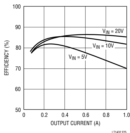
Figure 25. Positive-to-Negative Converter Efficiency
