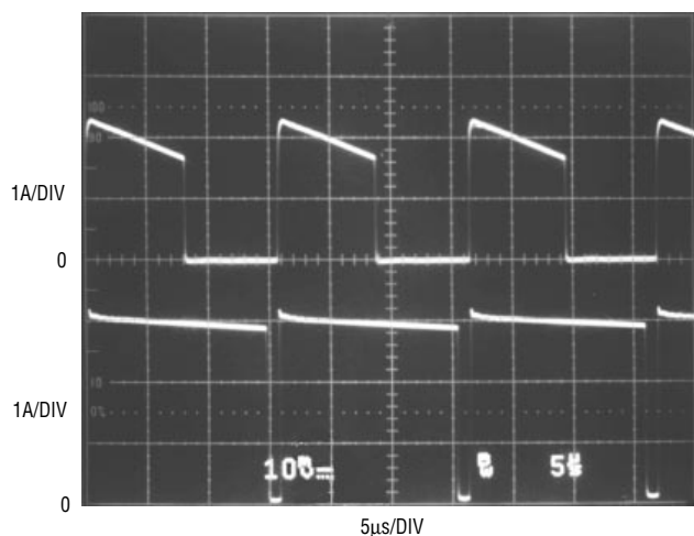
Figure 9. Diode Current
