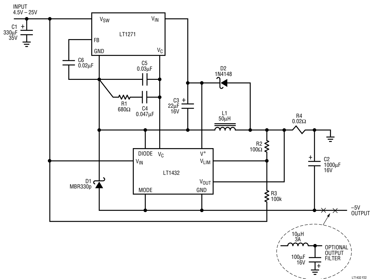
Figure 22. Positive-to-Negative Converter
