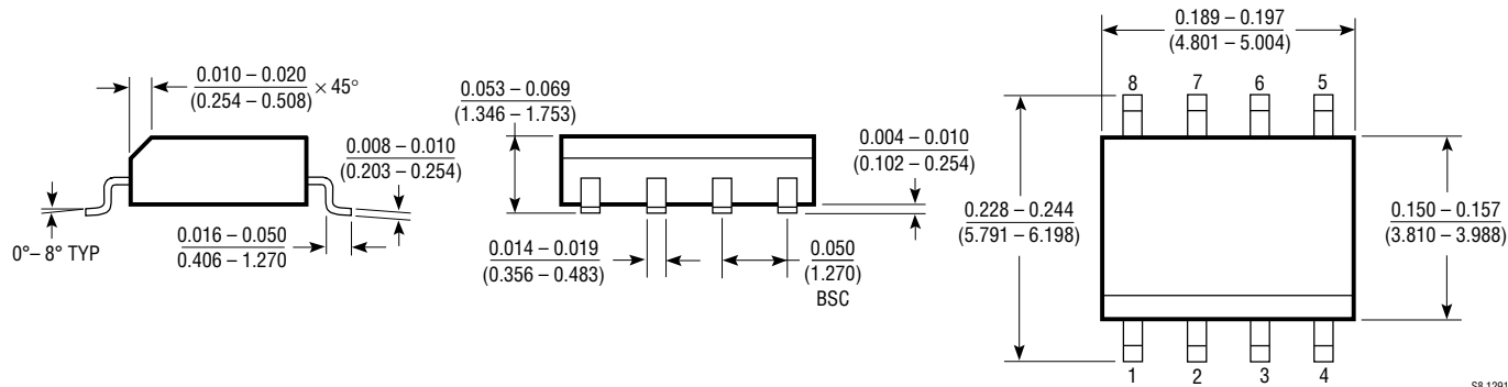
S8 Package 8-Lead Small Outline
