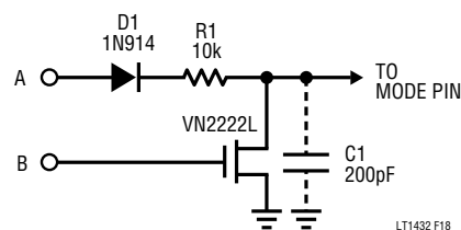
Figure 18. Two Input Mode Drive
